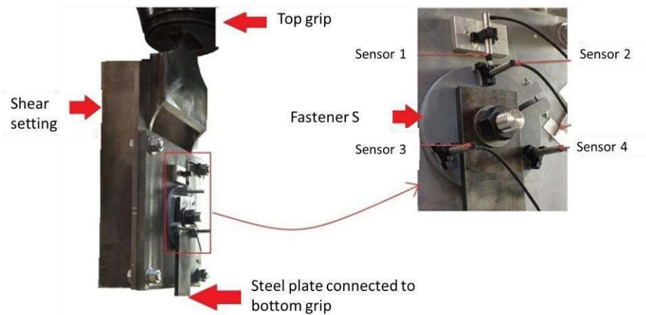
Fig. 7: Protocol of shear test.
