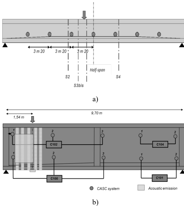
Fig. 6. Disposal of CASC sensors along the beam for flexure test (a) and shear test (b)
