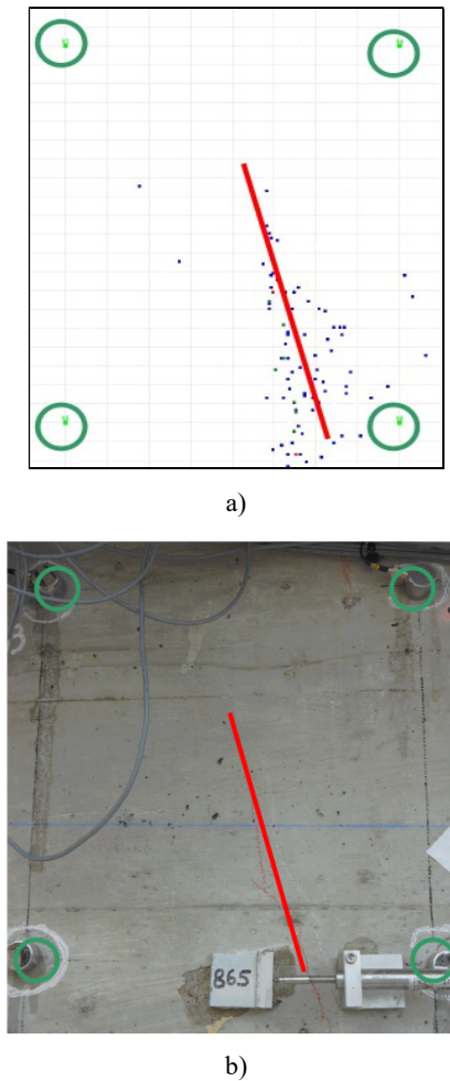
Fig. 8. Comparison of 2D events-localization (a) with visual crack identification at S4 section during initial tests (b)
