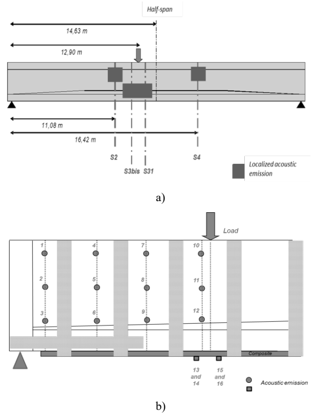
Fig. 7. Disposal of localized acoustic emission sensors for flexure test (a) and shear test (b)
