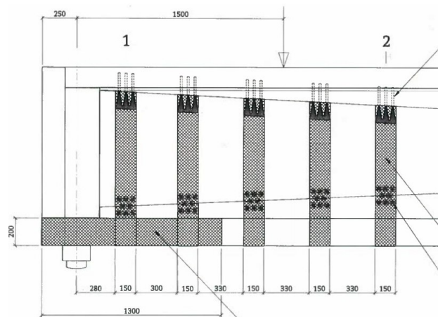
Fig. 5. Scheme of the shear reinforcement applied closed to the loaded end of the beam
