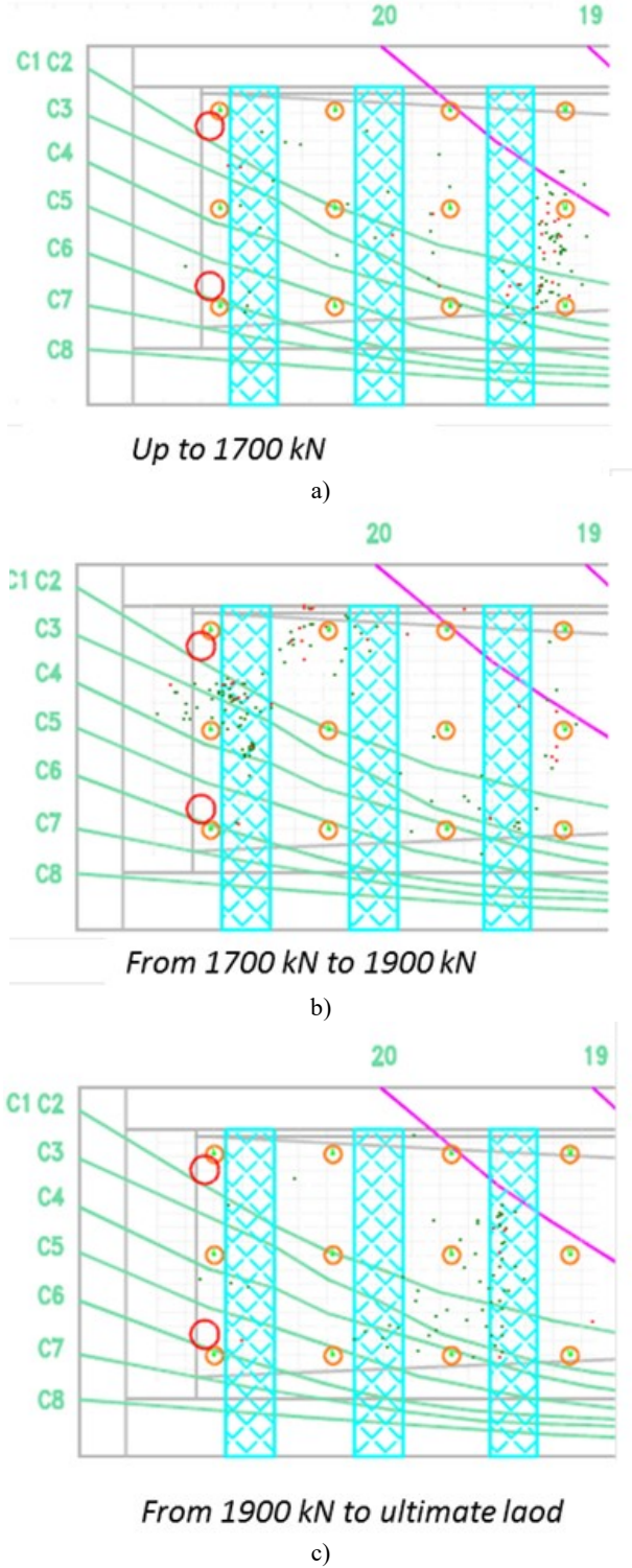
Fig. 14. Localized acoustic emission events during shear test up to failure (carbon sheets and prestressing cables are visualized) before 1 700 kN (a); between 1 700 and 1 900 kN (b) and from 1 900 kN to 1 970 kN corresponding to the ultimate load (c)
