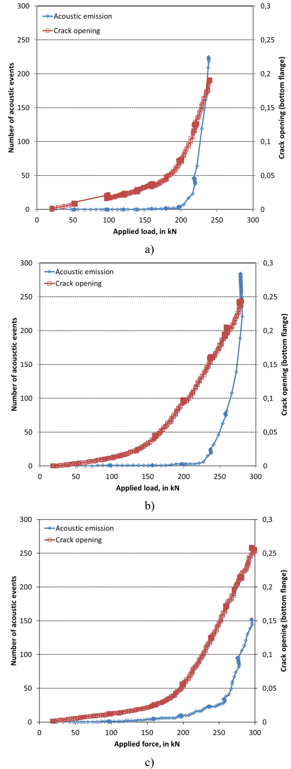
Fig. 9. Number of acoustic events and measured crack opening in function of the applied force before reinforcement (a), after first flexural reinforcement (b) and after final flexural reinforcement (c) at S4
