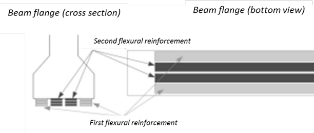
Fig. 4. Scheme of the flexural reinforcement applied on the beam flange
