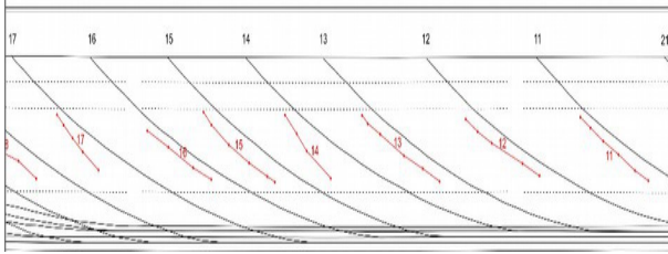
Fig. 2. Scheme of the prestressing cables position on one side of the beam
