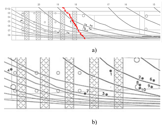
Fig. 15. 2D localization of acoustic events during shear test up to failure (whole beam with final crack: a; zoom on the events: b)
