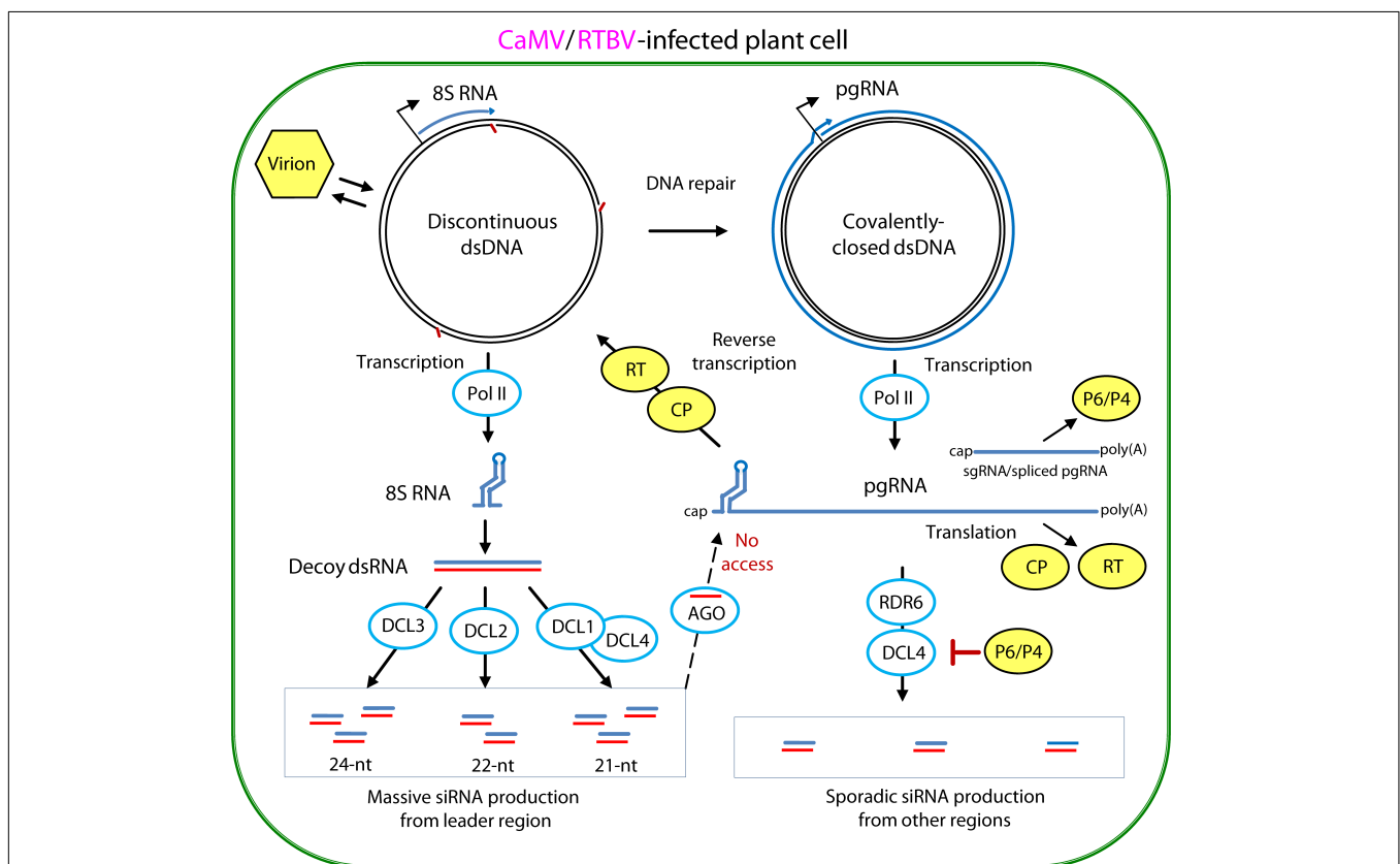
FIGURE 5 | Model for evasion and suppression of RNAi-based antiviral defenses in CaMV- and RTBV-infected cells. Viral DNA is released from the virion into the nucleoplasm. Gaps in the discontinuous dsDNA left after reverse transcription are repaired by the host repair enzymes to create covalently-closed dsDNA. Both repaired and unrepaired forms of viral dsDNA are transcribed by host Pol II. The repaired dsDNA gives rise to viral pgRNA, which serves as a polycistronic mRNA for CP and RT and a template for reverse transcription. In CaMV, Pol II transcription from a separate promoter generates subgenomic 19S RNA, mRNA for TAV/P6, while in RTBV, a fraction of pgRNA is spliced to generate mRNA for P4 protein. Abrupt termination of Pol II transcription at the minus-strand DNA gap (Met-tRNA gap) of the unrepaired dsDNA, results in production of 8S RNA. This RNA forms a viroid-like secondary structure which can be converted by Pol II to dsRNA. The resulting dsRNA serves as a decoy to engage all the four DCLs in massive production of 21-, 22-, and 24-nt viral siRNAs, which then get associates with AGO proteins. Stable secondary structure of the pgRNA leader sequence interferes with complementary interaction of viral siRNA-AGO complexes. The viral CP protein, which initiates packaging of pgRNA in pre-virions and assists its reverse transcription by RT within previrions, can also protect the pgRNA from being targeted by viral siRNAs. The CaMV protein P6 and RTBV P4 interfere with production of viral secondary siRNAs by the RDR6/DCL4 pathways. For further details, please, see the main text. Adapted from Pooggin (2016).
