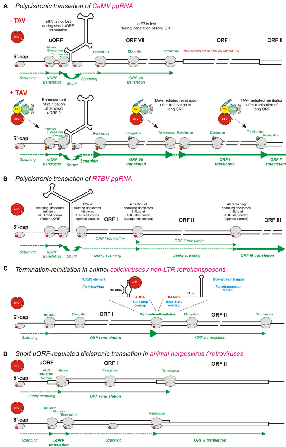
FIGURE 3 | Models for polycistronic translation in plant pararetroviruses CaMV and RTBV and in animal viruses and non-LTR retrotransposons. (A,B) Illustrate schematically the viral protein TAV-mediated reinitiation and the leaky scanning mechanisms operating on pgRNAs of CaMV and RTBV , respectively. (C) Illustrates the termination-reinitiation mechanisms operating in animal caliciviruses and non-LTR retrotransposons. (D) Illustrates the ribosomal sorting mechanisms operating in animal herpesvirus and pararetroviruses. eIF3 (red circle) is shown as the key initiation factor involved in polycistronic translation. Note that eIF3 alone or together with other factors is also shown in smaller scale on 40S or 60S ribosomal subunits (gray ovals). The CaMV TAV, through its interactions with eIF3, TOR, and RISP, keeps eIF3 attached to the translating ribosome during long ORF translation (see Figure 4 ) and thus promotes several consecutive reinitiations by post-terminating ribosomes. For further details, please, see the main text.
