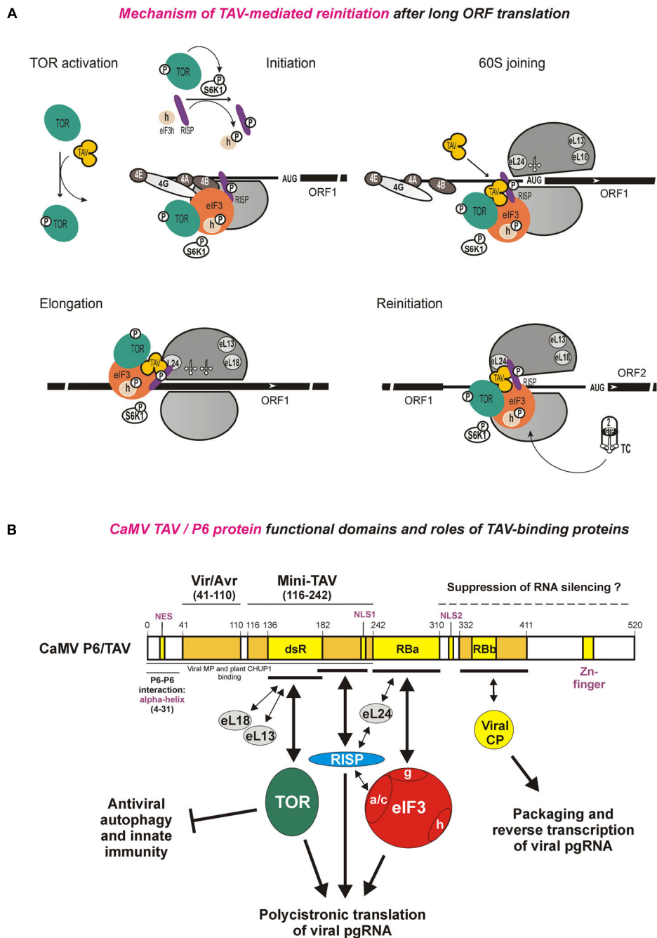
FIGURE 4 | Model for CaMV TAV function in reinitiation after long ORF translation and the functional domain structure of TAV protein with its interacting protein factors. (A) The mechanism of TAV-mediated translation reinitiation divided in five phases. At the TOR activation phase, TAV binds and activates TOR. At Initiation phase, activated TOR binds eIF3-40S preinitiation complex at the mRNA 5'-cap to trigger S6K1 and thus RISP and eIF3h phosphorylation. At 60S joining phase, eIF4B is replaced by TAV on eIF3, and TAV forms a complex with TOR-eIF3-RISP on 80S. During Elongation phase, TAV allows TOR-eIF3-RISP retention on the translating ribosome, through interaction with eL24 at the periphery of the 60S interface. At Reinitiation phase, following termination of long uORF translation, the putative TOR-eIF3-TAV-RISP complex is relocated back to 40S via eIF3-40S interactions. TAV and RISP bridge the 40S-bound eIF3 and the 60S-bound eL24, respectively, such that the post-terminating 60S remains attached to 40S and can be reused for the reinitiation event. The reinitiation-competent 40S-containing complex carrying 60S is capable of resuming scanning, rebinding a ternary complex (TC) and reinitiating at downstream ORF. eIF4E (4E), eIF4G (4G), eIF4A (4A), eIF4B (4B), eIF2 (2), tRNA and the ternary complex (TC, eIF2/GTP/Met-tRNA Met ) are indicated. Joining of TAV, recycling of TC and phosphorylation of S6K1 and RISP or eIF3h is shown by arrows. For further details, please, see the main text. Adapted from Thiébeauld et al. (2009), Schepetilnikov et al. (2011). (B) CaMV TAV interaction network illustrating functional domains of the TAV/P6 protein and roles of the TAV-binding cellular (TOR, RISP, eIF3, eL13, eL18, and eL24) and viral (CP and MP) proteins in polycystic translation and packaging/reverse transcription of CaMV pgRNA and in suppression of antiviral defenses. For further details, please, see the main text.
