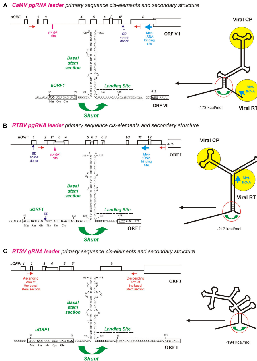
FIGURE 1 | Ribosome shunt configurations in the pgRNA leaders of pararetroviruses CaMV and RTBV and the genomic (g)RNA leader of picorna-like virus RTSV. (A–C) Show the primary sequence cis-elements and secondary structures of CaMV, RTBV, and RTSV pgRNA leaders, respectively. The leader-based multiple uORFs preceding the main long ORF are numbered and positions of the poly(A) signal, the splice donor (SD), and the Met-tRNA primer binding site are indicated. The large stem-loop secondary structure formed by the leader sequence is shown schematically on the right with binding sites for the viral proteins CP (coat protein) and RT (reverse transcriptase) indicated by yellow circles. A close-up of the shunt configuration (red circle) is shown of the left, with primary sequences of the 5'-proximal uORF1 followed by the ascending arm of the basal stem-section and the descending arm of basal stem-section followed by the shunt landing sequence. The nt numbering starts from the leader 5'-end. For further details, please, see the main text. Adapted from Pooggin et al. (1999,2012,2006).
