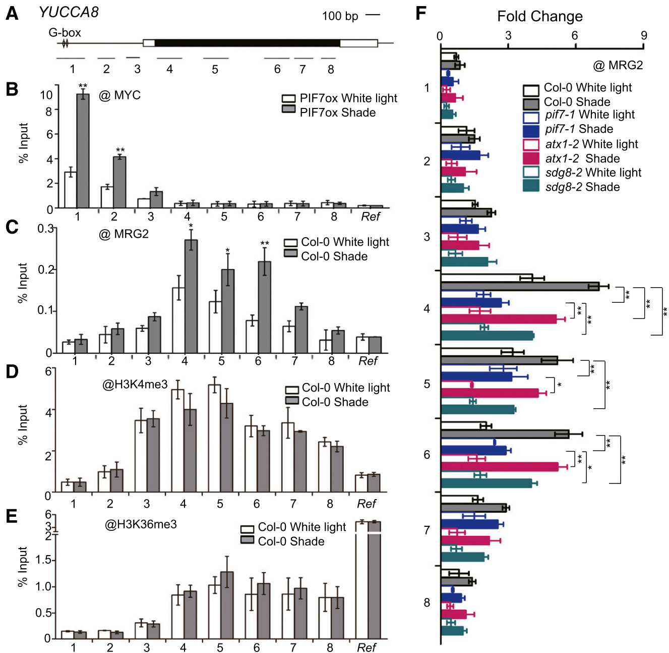
Figure 4. MRG2 and PIF7 bind chromatin at shade-responsive genes. A , Schematic of YUCCA8 gene structure. Black box represents the coding region, white boxes represent untranslated regions, and lines represent the promoter. The G-box elements within gene promoter are indicated. Bars underlabeled with numbers represent regions amplified by PCR. B , ChIP-PCR analyses using anti-MYC antibody at various chromatin regions of YUCCA8 in PIF7ox seedlings grown under white light and shade conditions. C , ChIP-PCR analyses using anti-MRG2 antibody at YUCCA8 chromatin in Col-0 seedlings grown under white light and shade conditions. D and E , ChIP-PCR analyses of H3K4me3 ( D ) and H3K36me3 ( E ) at YUCCA8 chromatin using Col-0 grown under white light and shade. F , ChIP-PCR analyses using anti-MRG2 antibody at YUCCA8 chromatin in the pif7-1 , atx1-2 , and sdg8-2 mutants as compared to Col-0 grown under white light and shade conditions. Seedlings were grown under white light for 4 d and maintained in white light or transferred to shade for 1 h ChIP and quantitative real-time PCR were performed using specific antibodies and gene primers, as indicated. A region of AT2G39960 served as an internal control and was used in normalization. Error bars represent \pm SE from three independent biological replicates. Asterisks in ( B ), ( C ), ( D ), and ( E ) indicate where the differences between white light and shade are statistically significant, and those in ( F ) indicate that the differences between two genotypes under shade are statistically significant ( *P < 0.05 , **P < 0.01 ). Ref, internal control.
