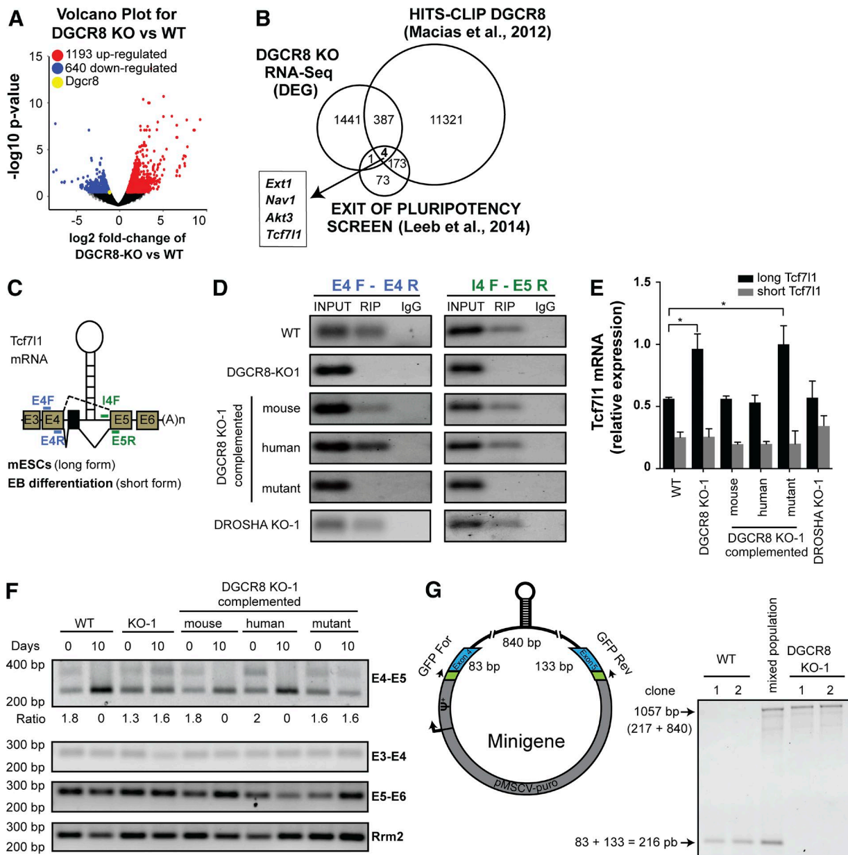
Figure 3. DGCR8 directly interacts with Tcf711 in a RNA-dependent manner and facilitates its alternative splicing. (A) Volcano plot showing the global transcriptional changes in Dgcr8_KO versus WT mESCs. The x axis shows the log fold change, and the y axis shows the -\log_{10} of the p-value. Differentially expressed genes are represented by colored circles and are defined by a fold change greater than two and a false discovery rate <0.1 . (B) Venn diagram showing the intersection between our RNA-seq, a DGCR8 HITS-CLIP (Macias et al., 2012), and a candidate list of exit from pluripotency genes (Leeb et al., 2014). (C) Exon structure graph for Tcf711 gene with differences in isoform expression between mESCs and EBs. The detected alternative exon is indicated as a black filled box. Dashed line between exons indicates an alternative splicing event. The hairpin structure in intron 4 is depicted as well. (D) DGCR8-immunoprecipitated RNA from WT, Dgcr8_KO , Droscha_KO , and complemented Dgcr8_KO mESCs. RIP was performed in triplicate, and a representative example is shown. INPUT, RNA isolated from input samples; RIP, RNA isolated from the immunoprecipitated DGCR8; IgG, RNA isolated from the immunoprecipitated IgG control. (E) Quantitative RT-PCR of long and short Tcf711 mRNA in WT, Dgcr8_KO , complemented Dgcr8_KO , and Droscha_KO mESCs. The data are shown as relative expression after normalization to the Rrm2 housekeeping gene. Error bars are the mean \pm SEM and are representative of three or more experiments. (F) RT-PCR of alternative splicing events in Tcf711 before (day 0) and after 10 d of differentiation (day 10). PCR amplicons from exons 3–4, exons 5–6, and Rrm2 were used as a control. Ratio: long Tcf711 /short Tcf711 . (G) Minigene splicing reporter analysis. Alternative splicing events in 1% agarose gel from independent single clones in WT and Dgcr8_KO mESCs. A mixed population of WT cells was used as a control. Representative gels of three or more experiments are shown. *, P < 0.05 ; Student's t test.
