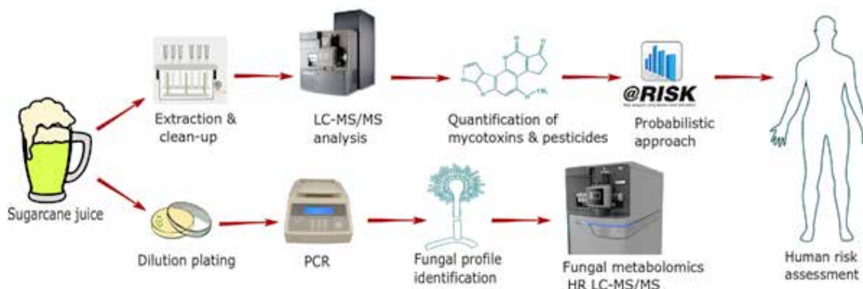
Figure 1: Proposed workflow to determine the commonly occurring mycotoxins in sugarcane juice. Food Frequency Questionnaires will be used to collect data for juice consumption in Egypt that will be used to conduct risk assessment studies. An untargeted approach will be used to screen and identify the unknown fungal secondary metabolites.
