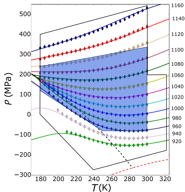
FIG. 1. Pressure along isochores. Symbols show simulations from the Princeton group of various isochores at the densities given on the right-hand side of the graph (in kg m -3 ). Solid lines of the same color represent the predictions of our TSEOS. The solid black line, open red circle, and dashed black line are the LLPT, LLCP, and Widom line, respectively. The dashed red line is the liquid-vapor spinodal. Isochores 960-1120 kg m -3 were first published in Ref. 17, while others are published here for the first time. All the data shown in this figure were included in the fit. The domains of validity of the previous 17 and present (extended) versions of TSEOS are shown with a shaded area and solid-line box, respectively.
