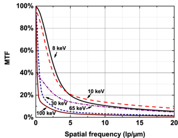
Fig. 3. Monte Carlo simulations of X-ray interaction MTF for a 3 \mu\text{m} LSO scintillator layer on a 167 \mu\text{m} LSO substrate at various X-ray energies. The MTF are derived from X-ray interaction PSF( r ) simulated within r \leq 50 \mu\text{m} from the X-ray beam.
