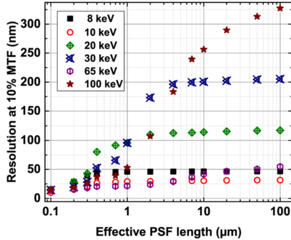
Fig. 4. Simulated spatial resolution expressed in nm at 10% MTF versus the length of X-ray interaction radial point spread function ( \sim X-ray pinhole diameter).
