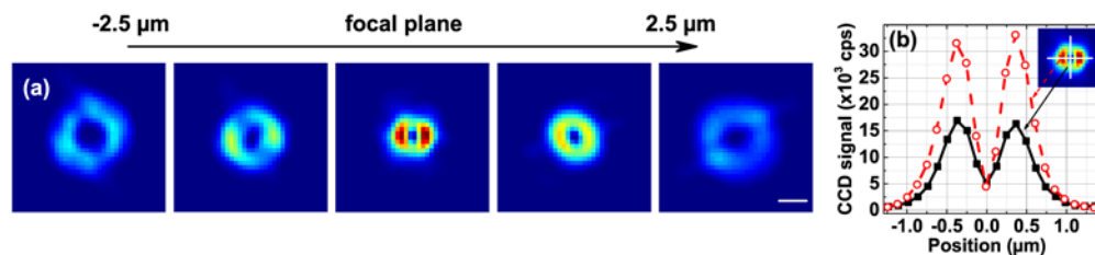
Fig. 5. STED-laser PSF measured as reflection of the STED-laser from the scintillator surface placed at various distances from the objective focal plane. Scale bar is 1 \mu\text{m} . (b) 1D STED-laser PSF intensity profiles measured along the lines in the inset of the figure.
