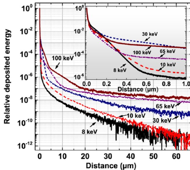
Fig. 2. Monte Carlo simulations of radial X-ray absorbed-dose distributions for various X-ray energies in a 3 \mu\text{m} LSO scintillator layer on a 167 \mu\text{m} LSO substrate.
