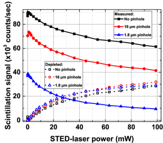
Fig. 6. (Solid curves) X-ray excited scintillation signal of LSO:Tb as a function of 628 nm STED-laser power. (Dotted curves) Depleted scintillation signal, derived as a difference between the original and the signal remaining under the depletion. The STED-laser power was measured before the objective and corrected for the objective transmittance.
