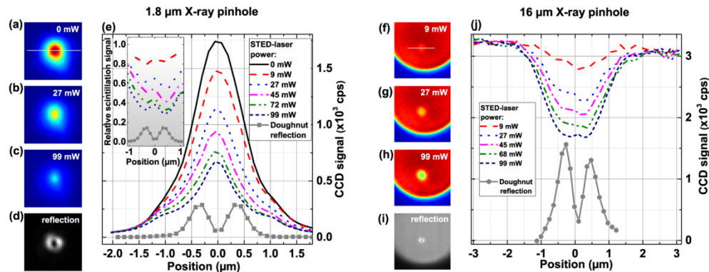
Fig. 7. Scintillation of LSO:Tb excited by X-rays passing through the 1.8 \mu\text{m} (a-e) and the 16 \mu\text{m} (f-k) X-ray pinholes measured with the CCD camera. (a-c) and (f-h) - 2D scintillation intensity maps at various STED-laser powers. (d,i) - reflection of the STED-laser doughnuts measured without the detection filters, in case of (i) - on top of the scintillation. (e,j) - 1D intensity profiles measured along the lines of Figs. (a,f).
