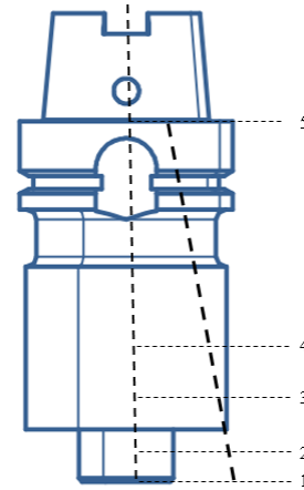
Figure 1. FRF measurement locations and assumed mode shape (black dash line) for the dummy tool.
