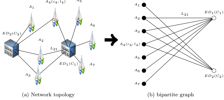
C_1 (resp. C_2 ) : total number of available CPU cores in BBU pool ED_1 (resp. ED_2 ) c_4 : number of CPU cores requested for processing the demands of antenna A_4 l_4 : expected latency for processing the demands of antenna A_4 L_{21} : communication latency on the fronthaul link between A_2 and ED_1
