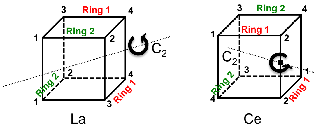
Figure 3. Representation of the ring 1 and ring 2, showing the orientation of the C_2 axis.
