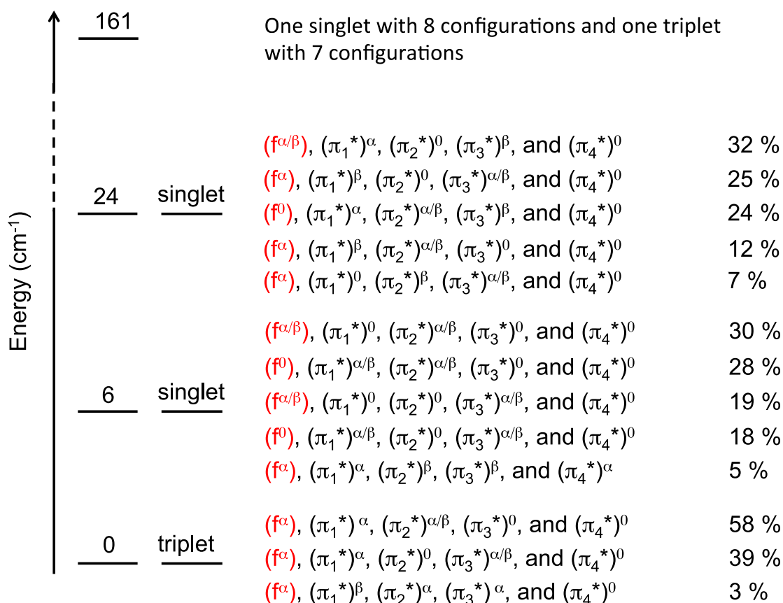
Figure 13. Energy levels and configuration of Yb (III, (f)^x ), (\pi_1^*)^a , (\pi_2^*)^b , (\pi_3^*)^c and (\pi_4^*)^d . All states show a nearly trivalent Yb, see main text.
