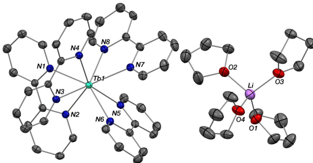
Figure 6. ORTEP of [Li(thf) 4 ][M(κ 2 -bipy) 4 ] Thermal ellipsoids are at 50 % probability. Carbon atoms are in grey, nitrogen atoms in blue, oxygen atoms in red, terbium in light green and lithium in purple.
