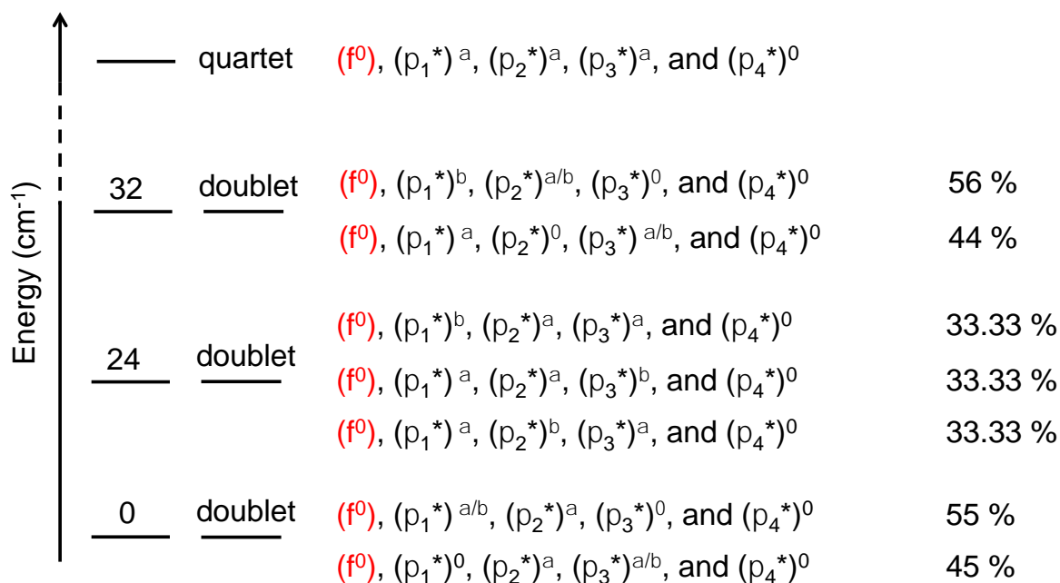
Figure 14. Energy levels and configuration of Lu (III, (f x ), (π 1 * ) a , (π 2 * ) b , (π 3 * ) c and (π 4 * ) d
