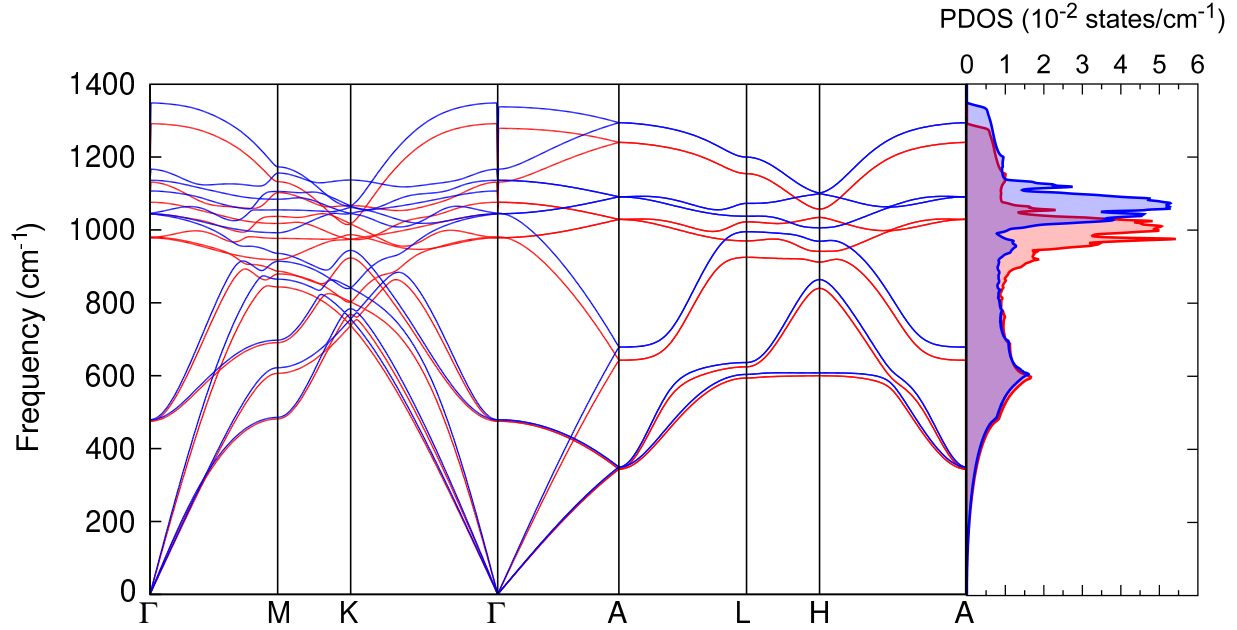
Figure 3: Phonon dispersion and phonon density of states of w -BN calculated using density functional perturbation theory at ambient pressure (red lines) and at 20 GPa (blue lines).
