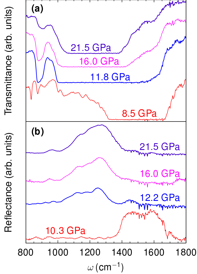
Figure 2: (a) IR transmission spectra of a BN sample recorded in the upstroke measurement at several pressures over the range where the h -BN \rightarrow w -BN transition takes place. (b) Reflectance spectra of a different BN sample at several pressures over the pressure range where the phase transition occurs.
