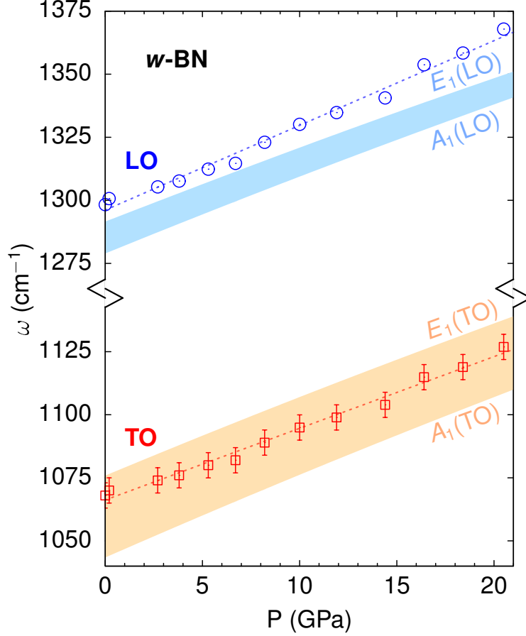
Figure 6: Pressure dependence of the TO (squares) and LO phonons (circles) of w -BN derived from the IR reflectance measurements. The error bars for the LO frequencies correspond to the size of the symbols. The dotted lines are linear fits to the data. The shaded areas indicate the region between the A_1 and E_1 frequencies of the TO (orange) and LO (cyan) modes obtained from ab-initio calculations.
