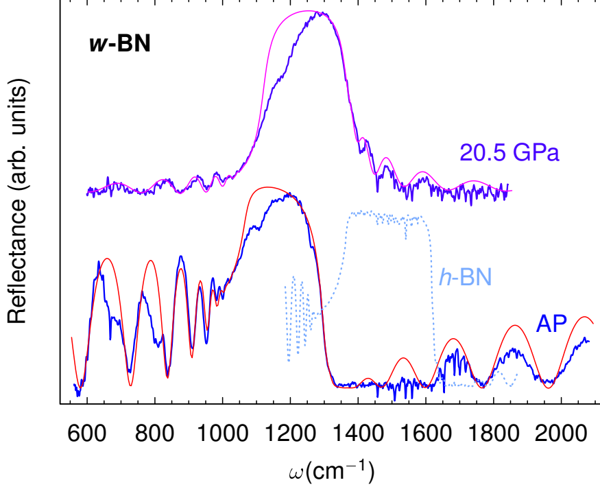
Figure 4: Reflectance spectra at normal incidence ( E \perp c ) of w -BN at 20.5 GPa and of the cold-compressed w -BN sample at ambient pressure outside the diamond anvil cell. The reflectance calculated using the dielectric model is displayed as magenta and red lines. For comparison, the reflectance spectra of the original h -BN crystal is also shown as a dotted line.
