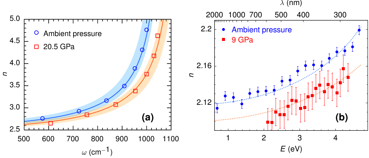
Figure 5: (a) Dispersion of the refractive index of w -BN close to the TO resonance at ambient pressure and at 20.5 GPa. The values obtained from the interference pattern are plotted with symbols and the values derived from the fit to the IR reflectance spectra are displayed as solid lines. The error bars at 20.5 GPa correspond to the size of the symbols, whereas at ambient pressure the error bars are about four times smaller. The shaded areas correspond to the region between the out-of-plane and in-plane refractive indices as given by the DFPT calculations. (b) Dispersion of the refractive index in the near-IR to UV spectral region at ambient pressure and at 9 GPa. The dotted lines are guides to the eye.
