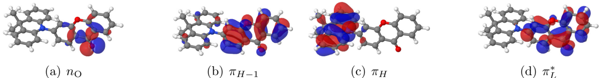
Figure 36: Frontier orbitals of ACRXTN at the optimised ground-state geometry.
