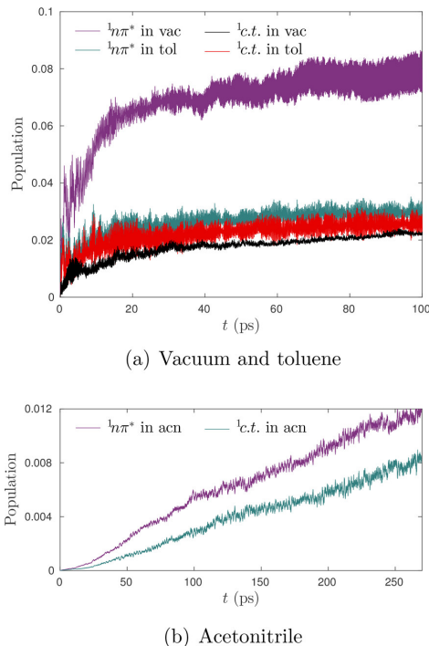
Figure 45: Time-dependent population of the singlet excited states of ACRSA in vacuum, toluene, and acetonitrile following the triplet CT exciton formation. Reproduced from ref. 149
