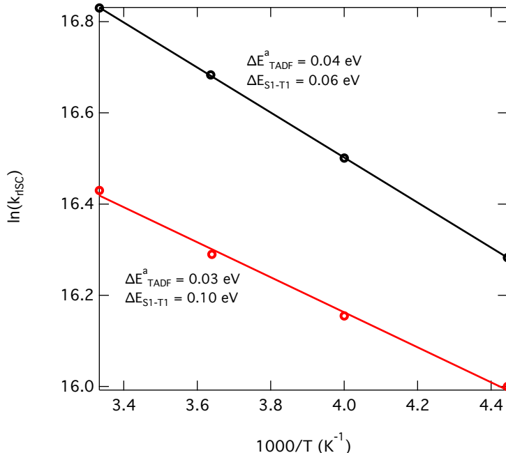
Figure 35: Energy barrier for TADF, determined from the temperature variation of k_{rISC} plotted against 1000/T (K -1 ) for two models which have \Delta E_{S_1-T_1} = 0.06 and 0.1 eV. In the case of the latter, the magnitude of nonadiabatic coupling has been doubled to enable these simulations to exhibit sufficient population transfer to S_1 at lower temperatures (225 K). Figure reproced from ref. 458
