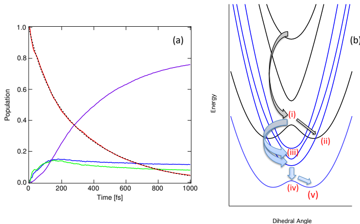
Figure 20: (a) Relative diabatic state populations of S_1 (blue), S_2 (green), S_3 (red), the triplet ( T_{1-4} ) states (purple), for 1 ps following photoexcitation. The black dashed line is the biexponential fit of the S_3 diabatic state populations. (b) Schematic representation of the key dynamical steps occurring within the ultrafast nonadiabatic dynamics of [\text{Cu}(\text{dmp})_2]^+ . (i) Internal conversion from S_3 to S_2 . (ii) Vibrational relaxation from S_1^{\text{FC}} to S_1^{\text{JT}} . (iii) Ultrafast ISC from S_1^{\text{FC}} to T_2^{\text{FC}} and T_2^{\text{FC}} . (iv) IC within the triplets. (v) Vibrational relaxation from T_1^{\text{FC}} to T_1^{\text{JT}} . FC is the Franck-Condon geometry and JT is the JT flattened geometry. Figures reproduced from ref. 154
