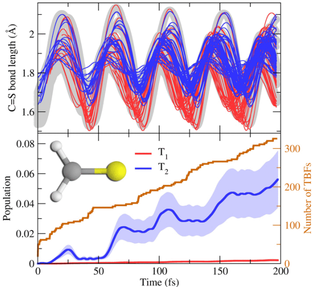
Figure 8: Dynamics of thioformaldehyde after photoexcitation to S_1 . Upper panel: C=S bond length for all basis functions. Basis functions are associated with the S_1 (light gray), T_1 (red), or T_2 (blue) electronic state. Lower panel: Population of the two triplet states during the dynamics (light area indicates the standard error). The total number of basis functions is given in orange. Figure reproduced from ref. 155
