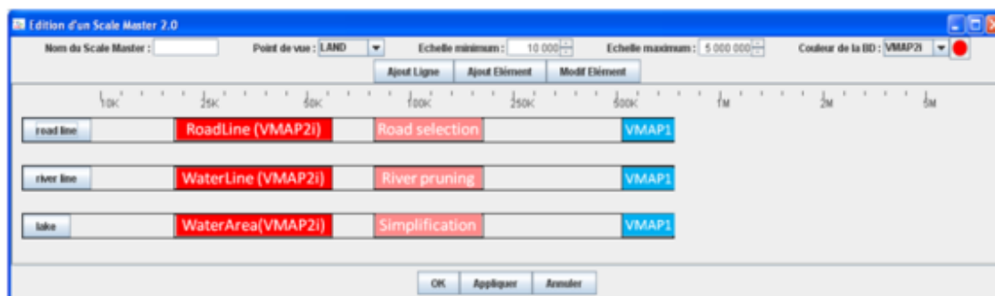
Figure 11. An interactive editor for the ScaleMaster2.0 model
