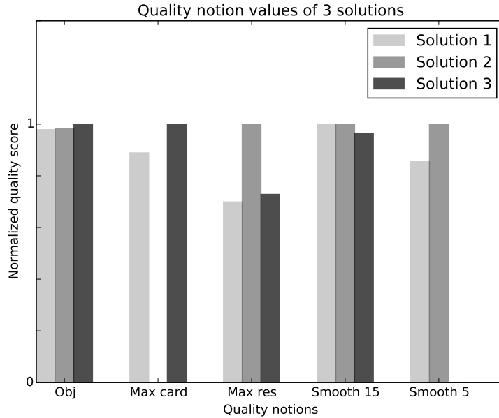
Figure 2: Three solutions of a GAP minimization problem: the scores of solutions are depicted according to the original objective value and four distinct quality notions. Note that solution 2 has a zero value for “Max card”, and solution 3 has a zero value for “Smooth 5”.
