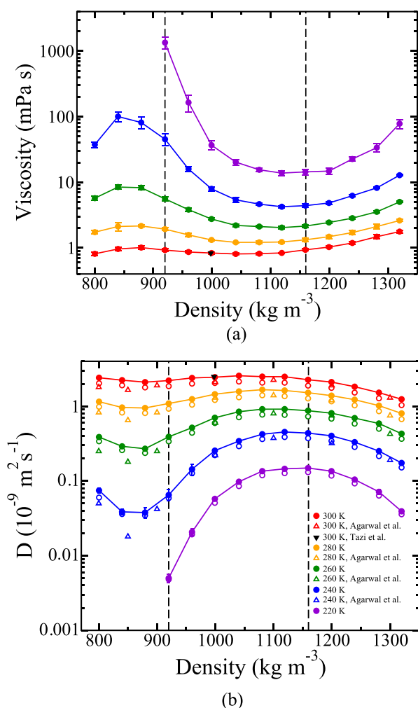
FIG. 1. Density dependence of viscosity (a) and self-diffusion coefficient (b) along several isotherms. The data set for each isotherm (circles: this work; down triangle: Ref. 28; up triangles: Ref. 17) is shown with a distinct color and labeled with the temperature in K. In (b), the empty and filled symbols correspond to data before and after correction with Eq. (1), respectively. The solid lines connecting points are guides to the eye. The vertical dashed lines bracket the validity region of the two-state model from Ref. 19.
