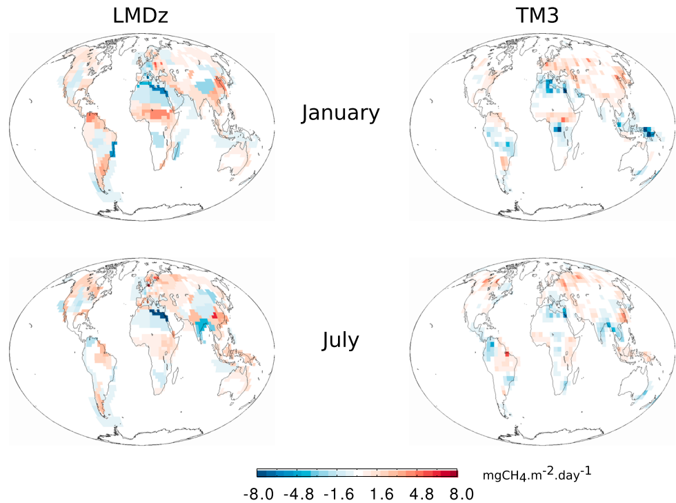
Figure 8. Comparison between LMDZ (left column) and TM3 (right column) for residual error statistics on methane emissions due to one scenario of systematic errors ( \text{mg CH}_4 \cdot \text{m}^{-2} \cdot \text{day}^{-1} ) for January (top row) and July (bottom row).
