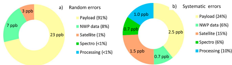
Figure 1. Relative share of contributors to the random error (a) and to the systematic error (b) for MERLIN XCH 4 . Note that the representation is linear (parts per billion in the pies), while the actual summation of contributors is quadratic (percentages in the legend). NWP = the Numerical Weather Prediction data used to perform the level 2 retrievals; Spectro = spectroscopy; MERLIN = MEthane Remote Lidar mission.
