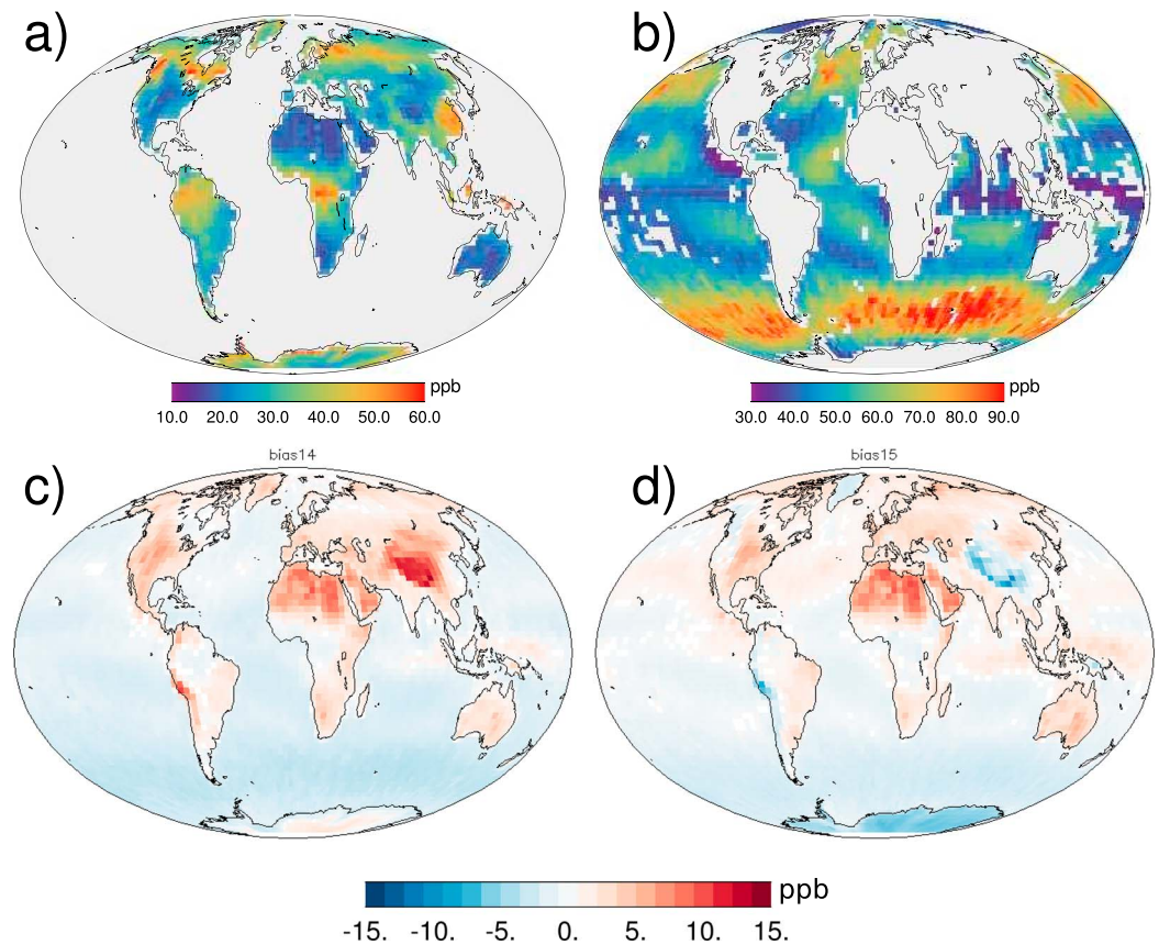
Figure 2. (a, b) Yearly average at 50 km of MERLIN random error for the methane atmospheric columns (ppb) for each LMDZ grid cell over continental regions (a) and over oceanic regions (b). Color scales are different between the two maps reflecting larger random errors over the oceans. (c, d) Two examples of scenarios for MERLIN systematic errors (ppb) with identical (c) or opposed signs (d) when combining albedo and surface pressure. All scenarios are presented in Figure S4b. MERLIN = MEthane Remote Lidar mission.
