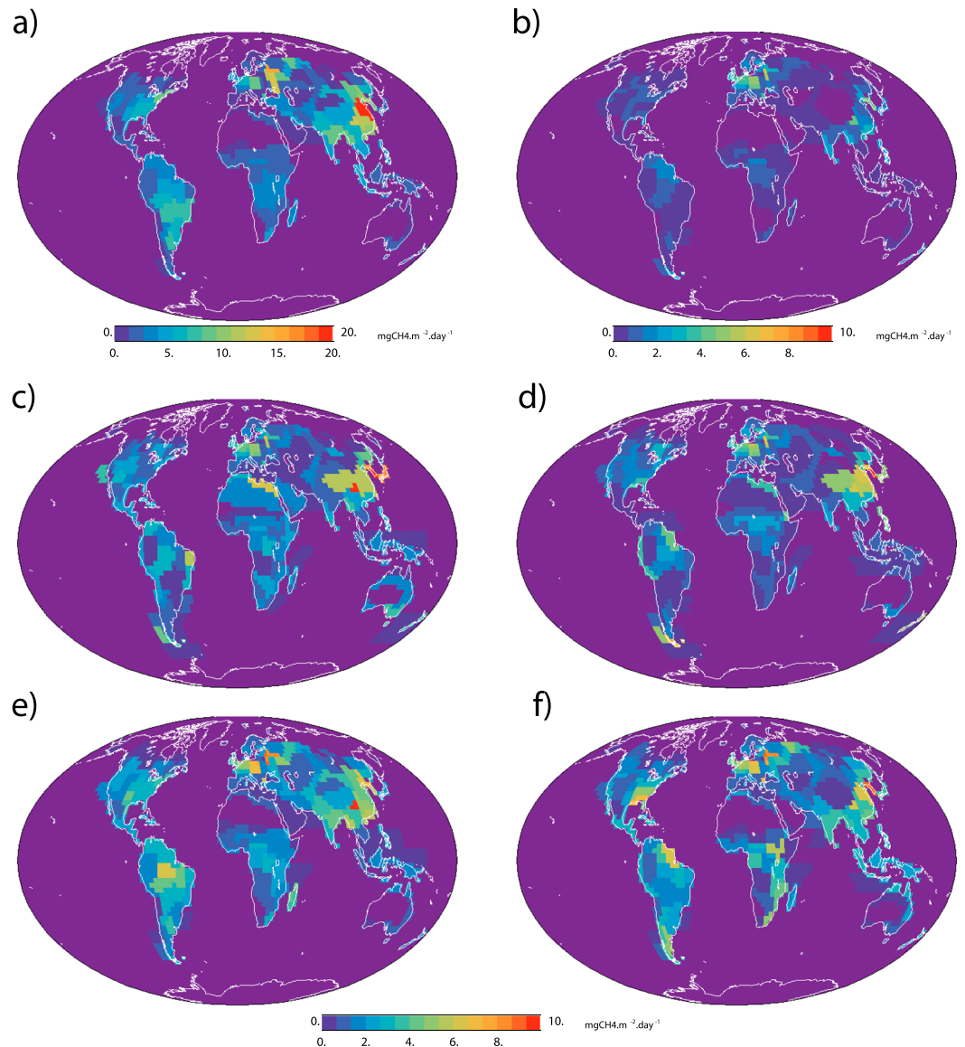
Figure 3. Errors on methane emissions ( \text{mg CH}_4\text{m}^{-2}\text{day}^{-1} ). (a) The prior random errors as injected in the OSSE ( \sigma_{\text{prior}} , B matrix, see section 3.2.1). (b) The residual random error \sigma_{\text{random}} as estimated by the OSSE. Maps (c) to (e) represent the total residual errors \sqrt{\sigma_{\text{random}}^2 + \beta_x^2} dominated by \beta_x for MERLIN scenario 14 (see section 3.2.2) in different configurations: All MERLIN data are assimilated (c), only MERLIN data over land are assimilated (d), and only MERLIN data over oceans are assimilated (e). (f) The residual systematic errors \beta_x for GOSAT scenario 14 (see section 3.3). MERLIN = Methane Remote Lidar mission; OSSE = Observing System Simulation Experiments; GOSAT = Greenhouse Gases Observing Satellite.
