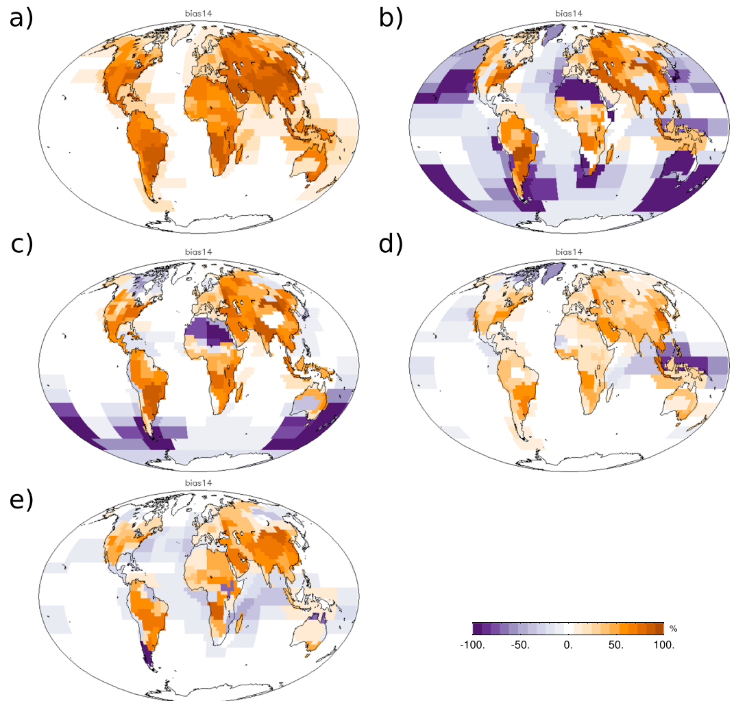
Figure 4. Example of uncertainty reduction E_{red} (%) (see equation (4)) on methane emissions when only random errors are taken into account (a) and for the same three configurations of systematic error scenario 14 as shown in Figure 3 (b, c, d). (b) All MERLIN data are assimilated. (c) Only MERLIN data over land are assimilated. (d) Only MERLIN data over oceans are assimilated. (e) All GOSAT data are assimilated. A negative uncertainty reduction indicates regions where systematic errors lead to larger uncertainties than the current uncertainty on surface emissions. Contributions of the different regions to the global methane emissions are shown in Figure 7 and printed in Table 3. Residual uncertainties on emissions for all scenarios are presented in Figures S4d (MERLIN) and S4e (GOSAT). MERLIN = METHane Remote LIdar mission; GOSAT = Greenhouse Gases Observing SATellite.
