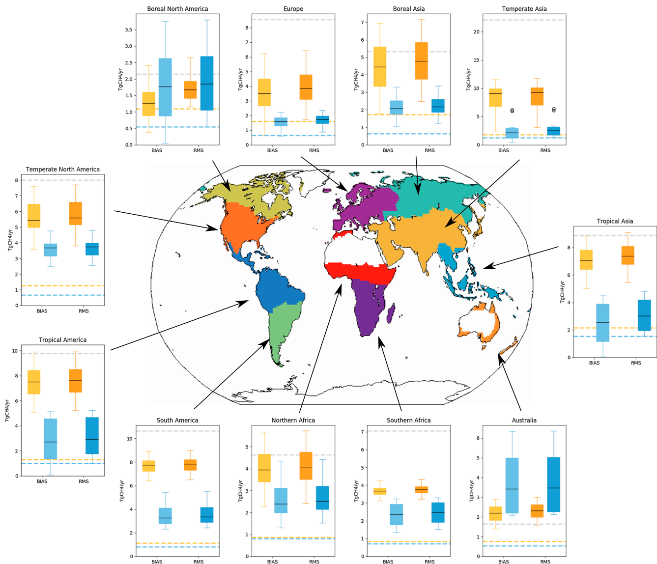
Figure 5. Posterior error statistics of regional methane emissions for MERLIN and GOSAT ( \text{Tg CH}_4/\text{year} ) using SIMGHG. For 11 continental regions, a comparison between residual errors on methane emissions between MERLIN (blue) and GOSAT (orange) is proposed: Dark blue/orange boxplots (the two rightmost boxplots of each region) represent the MERLIN/GOSAT residual total error (RMS), light blue/orange boxplots (the two leftmost boxplots of each region) represent the MERLIN/GOSAT residual systematic error, and dashed blue/orange lines are the MERLIN/GOSAT residual random error. The prior error is shown as the dashed gray lines. The box extends from the lower to upper quartile values of the data, with the median values shown in black; the whiskers show the range of the data between the first and third quartiles \pm 1.5 times the interquartile range. White continental areas correspond to desert zones of Australia and Sahara that have been removed from the analysis (see text). MERLIN = MEthane Remote Lidar mission; GOSAT = Greenhouse Gases Observing SATellite; RMS = root-mean-square; SIMGHG = OSSE system based on LMDZ model (see section 2).
