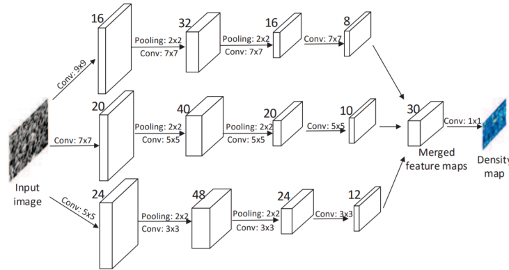
Fig. 1. The structure of network proposed in (Zhang et al., 2016).
