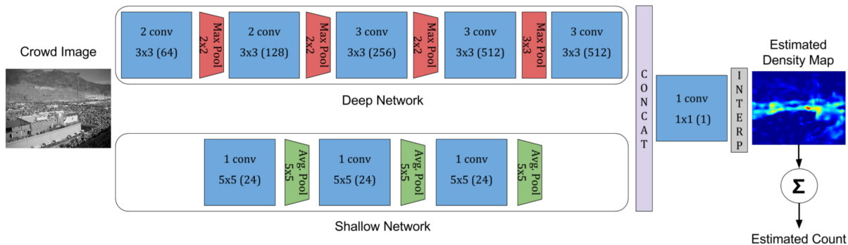
Fig. 2. The structure of network proposed in (Boominathan et al., 2016).
