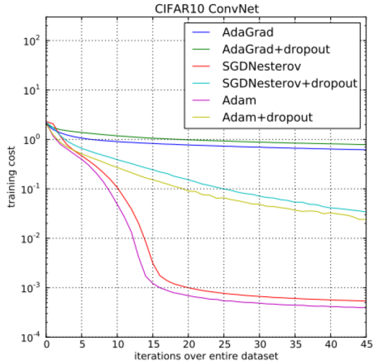
Fig. 6. Convolutional neural networks training cost for CIFAR10 deep architecture over 45 epochs (from Kingma and Ba (2015)).
