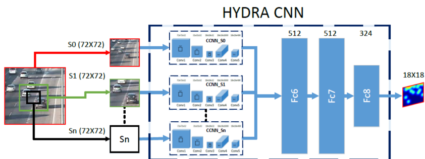
Fig. 3. The structure of network proposed in (Onoro-Rubio and López-Sastre, 2016).
