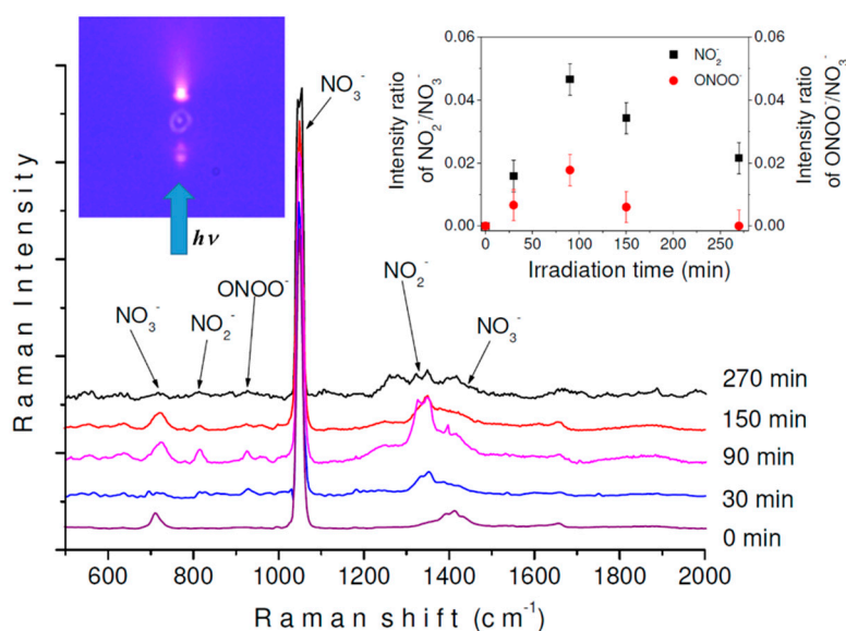
Figure 5. Raman spectra of a microdroplet of aqueous \text{NaNO}_3 obtained after different times of UV light irradiation ( 254 \pm 25 nm) using an excitation line of 532 nm. (Left inset) Photograph of top capture of the particle during the irradiation process. (Right inset) Intensity of \text{NO}_2^-/\text{NO}_3^- and \text{ONOO}^-/\text{NO}_3^- ratios as a function of the irradiation time.
