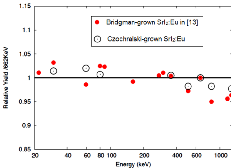
Fig. 6. Non-proportionality of Czochralski-grown SrI 2 :Eu using various typical radioactive sources vs. Bridgman-grown SrI 2 :Eu in [13]. The values are normalized by the light yield at 662 keV.
