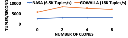
Figure 8: Parallel PINED-RQ++
