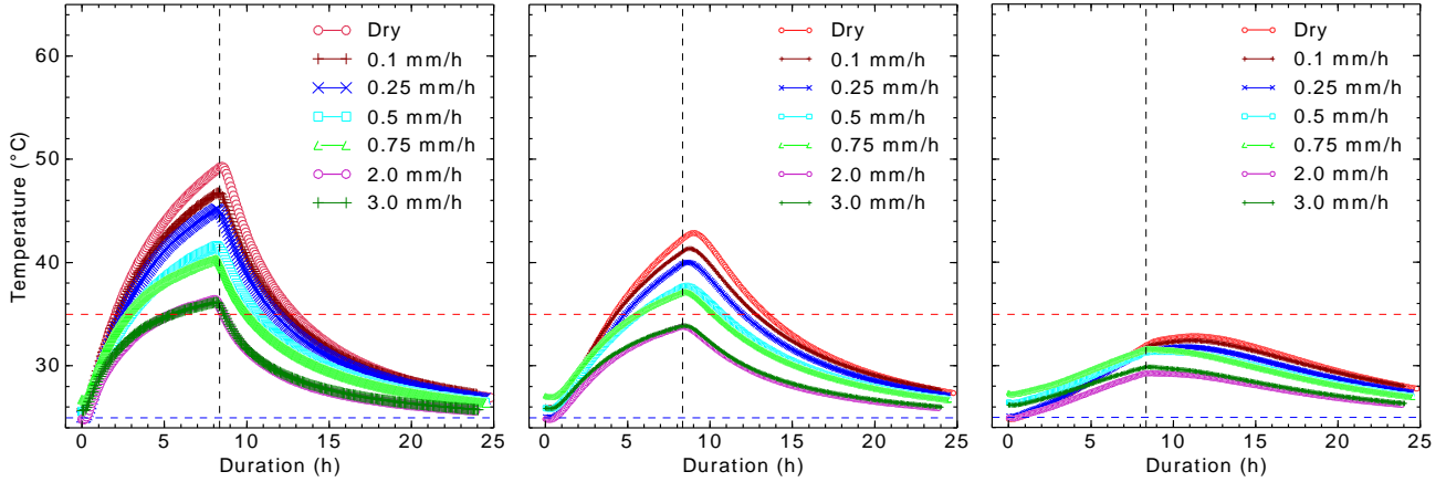
Figure 7: Temperature variations 6 cm (left), 14 cm (center) and 25 cm (right) deep for non-watered and watered trials (i.e. 0.1, 0.25, 0.5, 0.75, 2.0 and 3.0 mm/h)
