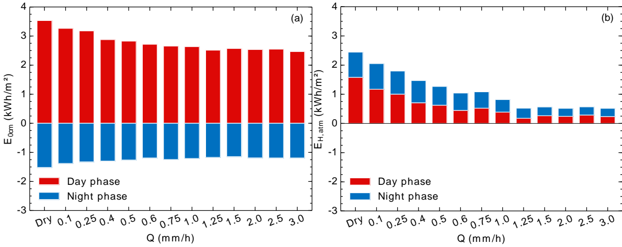
Figure 12: Stored (day phase) and released (night phase) pavement surface conduction energy density, E_{0cm} (a), and released (day and night phases) atmospheric convective energy density, E_{H, atm} (b), to watering rate.
