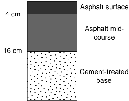
Figure 1: Studied structure sample
