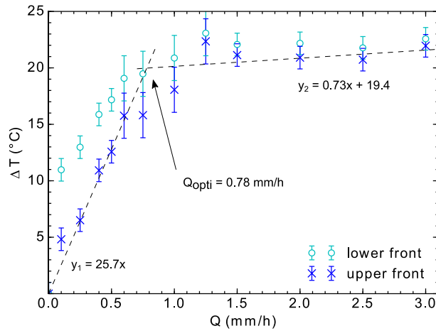
Figure 6: Difference between non-watered and watered maximum surface temperature \Delta T_{max}^{dry-wet} for lower and upper fronts as a function of the watering rate. A double linear piecewise regression with zero-intercept is used (dashed lines) to distinguish the two regimes.
