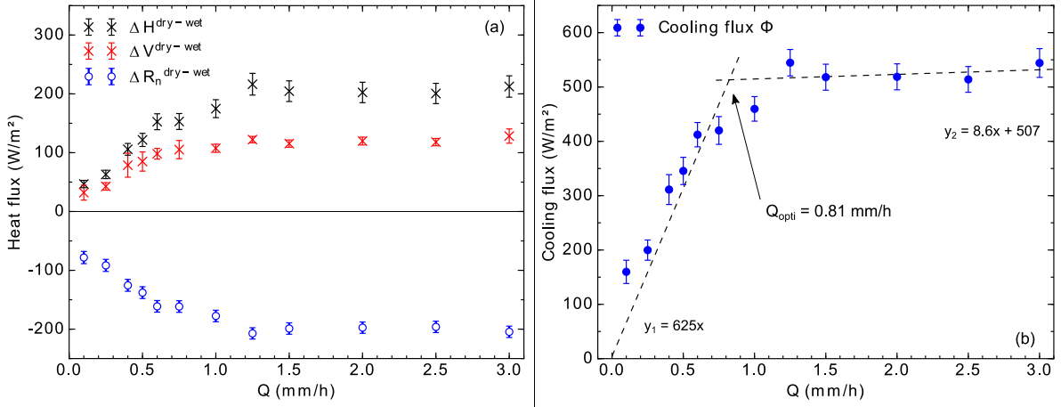
Figure 13 : Net radiation dry-wet difference \Delta R_n^{dry-wet} , absorbed surface heat flux dry-wet difference \Delta V_{0cm}^{dry-wet} and convective heat flux dry-wet difference \Delta H^{dry-wet} (a), and pavement cooling flux \Phi (b) to watering rate Q at the end of day phase. A double linear piecewise regression with zero-intercept is used on \Phi (b) (dashed lines).
