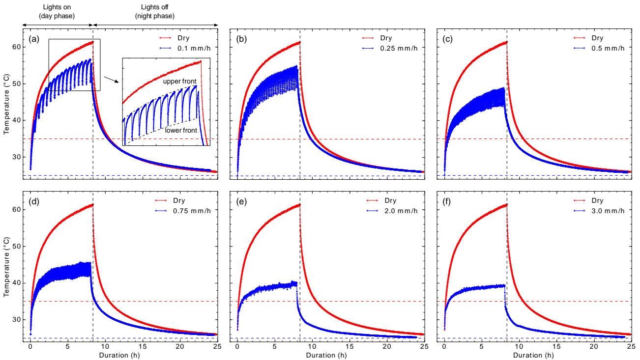
Figure 4: Surface temperature variations of the asphalt road sample with (blue) and without (red) watering for various watering rates (namely 0.1 (a), 0.25 (b), 0.5 (c), 0.75 (d), 2.0 (e) and 3.0 (f) mm/h). Horizontal dashed lines respectively represent day (red) and night (blue) phases air temperature, while the black vertical dashed line marks the transition between day and night phases.
