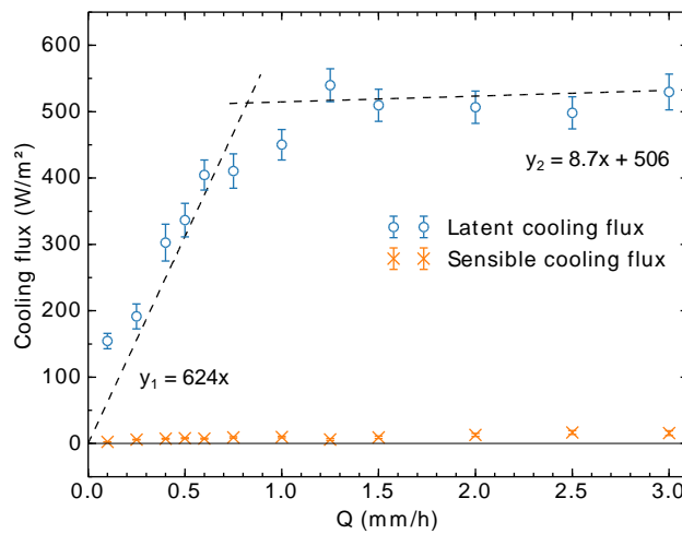
Figure 14: Latent and sensible cooling flux, \mathcal{L}E and \Phi_{sens} respectively, to watering rate.
