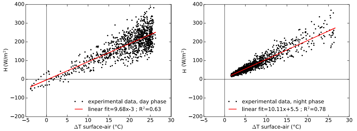
Figure 11: Convective heat flux during the day phase (left) and the night phase (right), both fitted using a linear regression.
