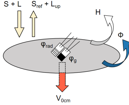
Figure 3: Schematic diagram of heat balance at the pavement surface. S is downward shortwave (SW) radiations, L longwave (LW) radiations, S_{ref} and L_{up} , respectively the reflected SW and upward LW radiations, H the upward atmospheric convective heat flux, V_{0cm} the absorbed heat flux at the surface, \Phi the cooling flux due to watering. \varphi_{rad} is the radiative flux measured by a radiative heat flow sensor ( \varepsilon=1 , \alpha=0 ) and \varphi_g the global heat flux measured by the fluxmeter ( \varepsilon=0.95 , \alpha=0.05 ).
