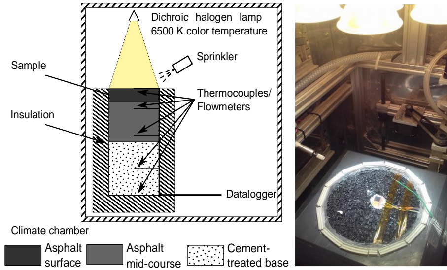
Figure 2: Diagram (left) and photograph (right) of the experimental set-up
