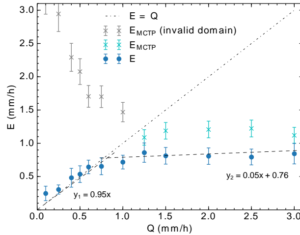
Figure 15: Evaporation rate of the water-film sprinkled during the day phase as a function of the watering rate.
