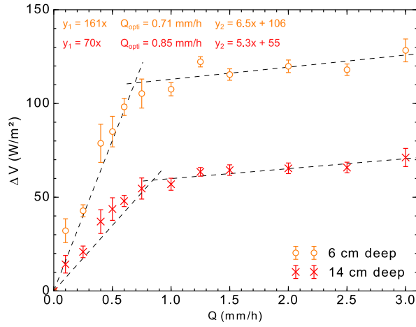
Figure 10: Average day-phase difference between dry and watered conduction heat flux to watering rate, for 6 and 14 cm deep signals.
