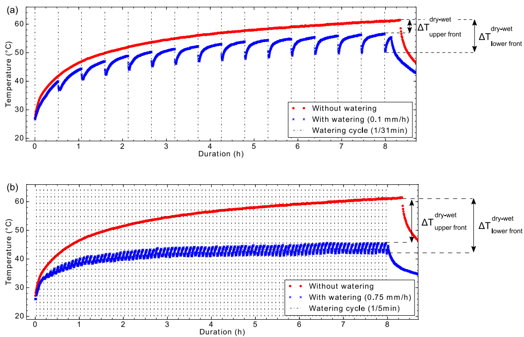
Figure 5: Asphalt road surface temperature during day phase with (blue) and without (red) watering, for 0.1 mm/h (a) and 0.75 mm/h (b).
