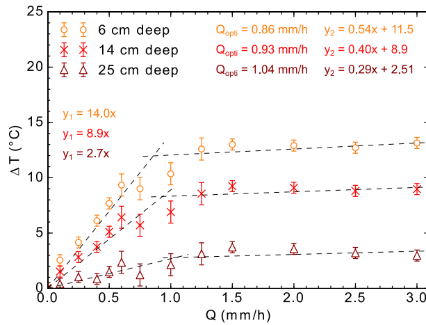
Figure 8: Difference between non-watered and watered maximum in-depth temperatures \Delta T_{max}^{dry-wet} 6 cm, 14 cm and 25 cm deep as a function of the watering rate. Best double piecewise fits for both regimes and each depth are illustrated with dashed lines.
