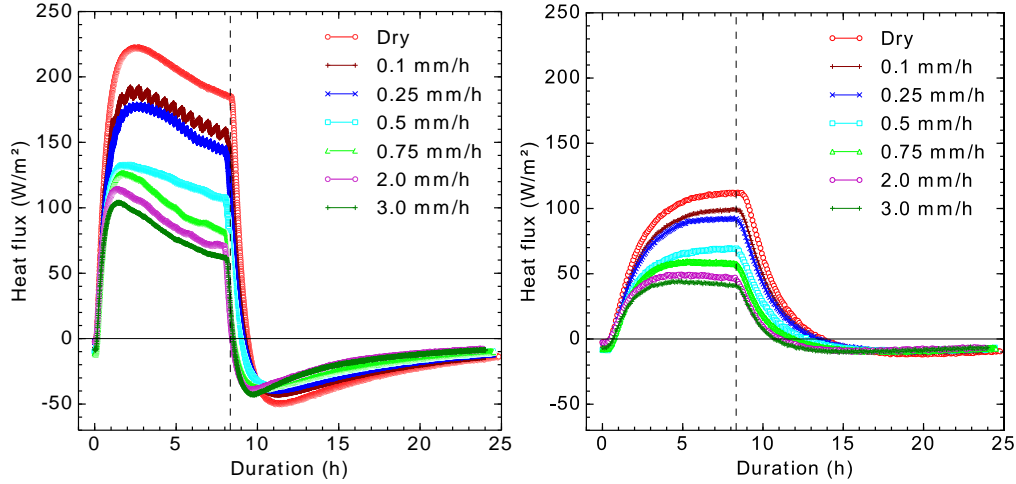
Figure 9: Conduction heat flux 6 cm deep (left) and 14 cm deep (right) for a dry and watered trials (0.1, 0.25, 0.5, 0.75, 2.0 and 3.0 mm/h)
