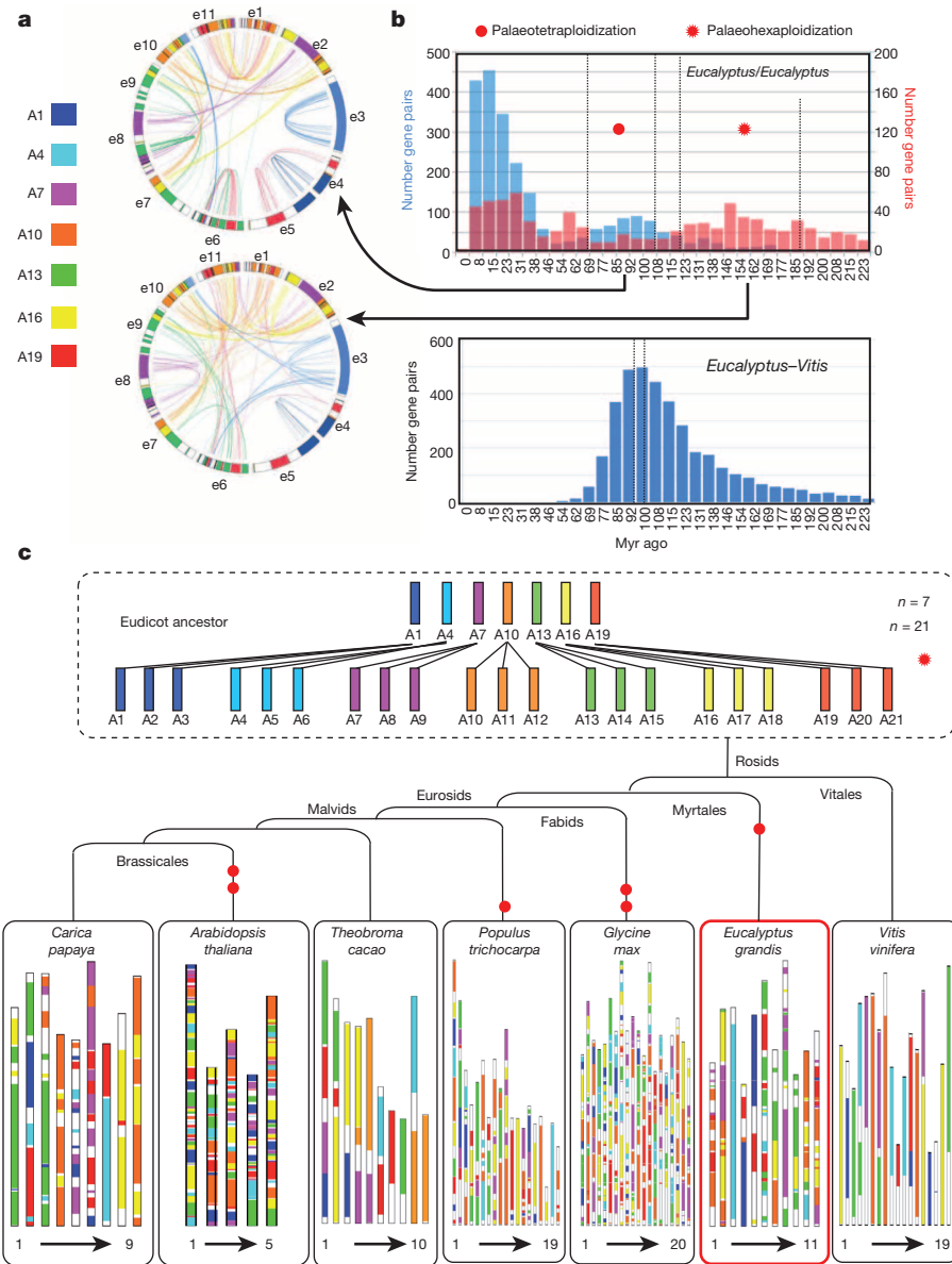
Figure 2 | Eucalyptus grandis genome synteny, duplication pattern and evolutionary history.
