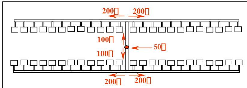
Figure 5 : 24 \square 2 antenna array
