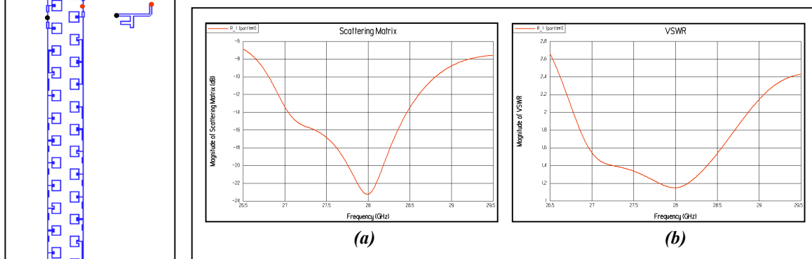
Figure 7 : Return loss and VSWR referenced to 50Ω
