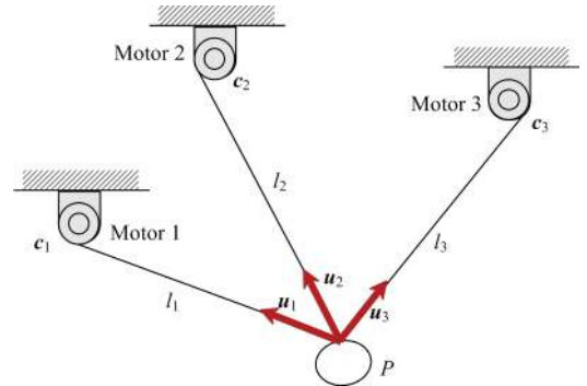
Fig. 8 Diagram of kinematic parameters.
