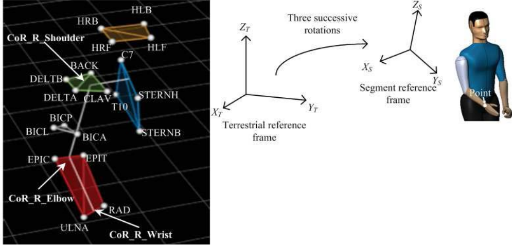
Fig. 5 Reconstruction of several detected markers into segments: arm, forearm and torso.
