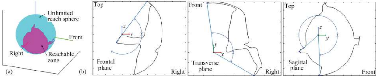
Fig. 6 (a) Shoulder range of motion for extended arm; (b) RoM projection on frontal, transverse and sagittal planes.
