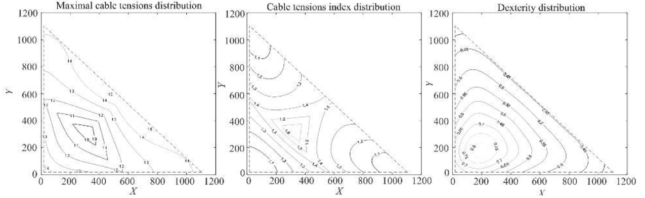
Fig. 13 (a) Distribution of maximal cable tensions in daN; (b) distribution of the cable tensions index; (c) distribution of dexterity index for a given high z = 1000 in (x, y) plane.
