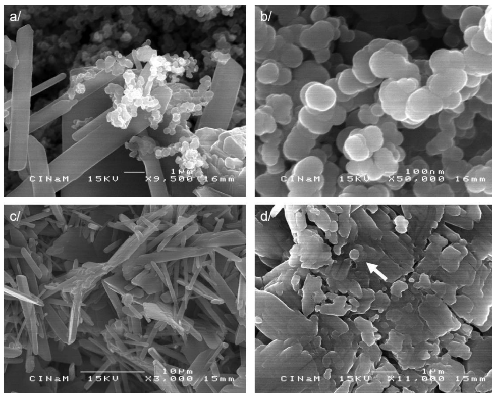
Figure 5. SEM micrographs of gypsum covered with lamp black before (Area 1) and after Q-S laser cleaning (Area 2) obtained in secondary electron mode. a/ Surface of the plaster plate showing gypsum crystals covered with aggregates of lamp black particles (Area 1). b/ Aggregates of lamp black particles of spherical shapes (Area 1). c/ Surface of the plate after Q-S laser cleaning (Area 2). d/ Details of the gypsum crystal where some alterations are observed (Area 2).
