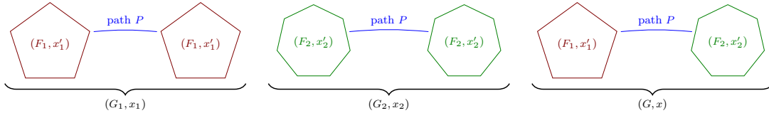
Fig. 2: Illustration of the “cutting and gluing” construction of (G, x) from (G_1, x_1) and (G_2, x_2) .
