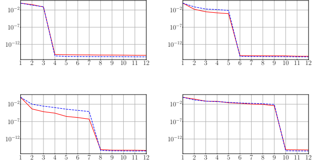
Fig. 2. First singular values of \mathbf{M}_3 (red) and \mathbf{M}_2 (blue) (Top-left: R = 3 , Top-right: R = 5 , Btm-left: R = 7 , Btm-right: R = 9 )
