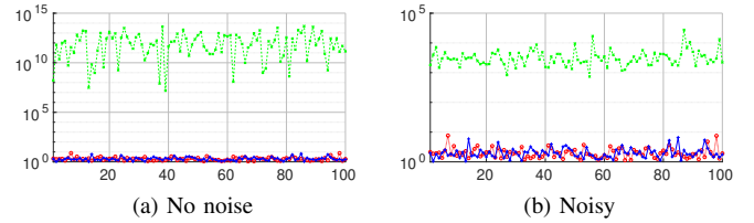
Fig. 3. Singular value ratios gap of \mathbf{M}_2 for 100 tests (In red: \sigma_5/\sigma_6 , in blue: \sigma_6/\sigma_7 , and in green: \sigma_7/\sigma_8 )
