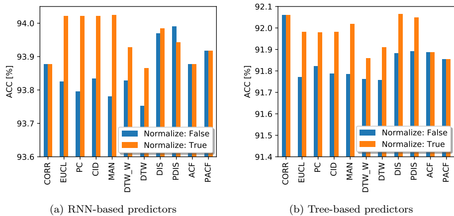
Fig. 9 Impact of time-series values standardization
