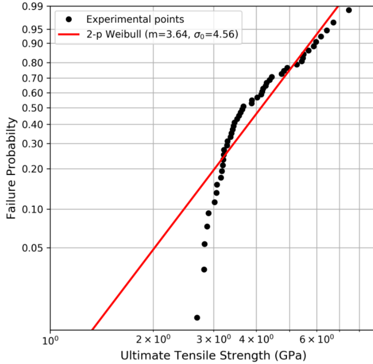
Figure. 1. Weibull plot with 50 fibre strength data points for T700 carbon fibres (Determined at Dia-Stron Ltd.).
