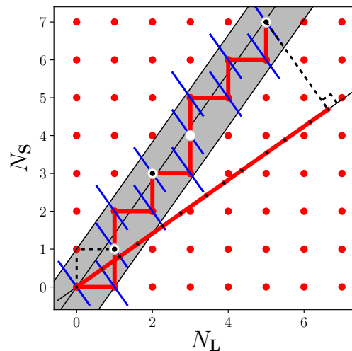
FIG. 6. Strip and projection method to generate a \sqrt{2} -tiling from the square lattice. The gray strip has a slope equal to \sqrt{2} fixing the ratio N_S/N_L = \sqrt{2} . The lower limit of the strip goes through the point (1, 0) and the upper limit through (0,1). The strip is half-bounded with the upper limit excluded here. The square edges and the sites of the square lattice inside the strip are selected. Once projected onto a straight line, they correspond respectively to the tiles and vertices of the tiling. If projected onto a line of slope \sqrt{2} identical to the slope of the strip, the length of the segments would be in the ratio P_L/P_S = 1/\sqrt{2} . To get the ratio P_L/P_S = \sqrt{2} , they are projected onto a line of slope 1/\sqrt{2} . The equivalence with the cut method is also sketched: a line segment is periodically set on every site of the lattice (for clarity only those selected by the strip are drawn). The vertices of the tiling are now the intersection points between all segments and the line of slope \sqrt{2} going through the origin. To get the correct length ratio, the segments are perpendicular to the line with slope 1/\sqrt{2} . The common length of the segments is the width of the strip along this direction. The white disks inside the strip correspond to the best rational approximations N_S/N_L of \sqrt{2} , i.e. |N_S/N_L - \sqrt{2}| < |p/q - \sqrt{2}| , \forall q \leq N_L . Among them, those with a central black dot correspond to the continued-fraction convergents, which are solutions of the stronger condition Eq 1.
