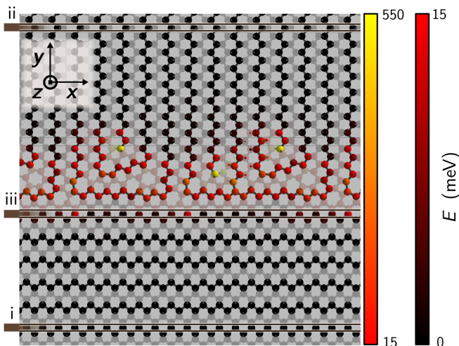
FIG. 9. Atomic-configuration visualization highlighting the calculation of the hull functions \Delta x and \Delta y plotted in figure 10. Only one atomic layer perpendicular to z is not shaded by a transparent mask. Far from the interface, the atoms selected by the two lowest horizontal lines are representative of a crystalline atomic row, i , of grain I. In the same way, the two highest horizontal lines correspond to an atomic row, ii , of grain II. At the interface, the horizontal lines correspond to an atomic row, iii , that has been chosen for calculating its hull plots. Any atomic row could be selected, however this one is the closest to the interface with atoms having the same first-neighbor environment than those of grain I. That way, the influence of grain II on grain I can be analyzed. The opposite would be possible by choosing an atomic row in grain II. To simplify the discussion, row i has been chosen to select crystallographically equivalent lattice sites than those of row iii . The atomic configuration has been relaxed with the Stillinger-Weber potential 23 to get atomic energies. These energies are color coded with two successive color gradients. From zero to 15 meV, the first scale shows the energy range in rows iii . From 15 meV to 550 meV, the second scale highlights the high energy spots at the interface.
