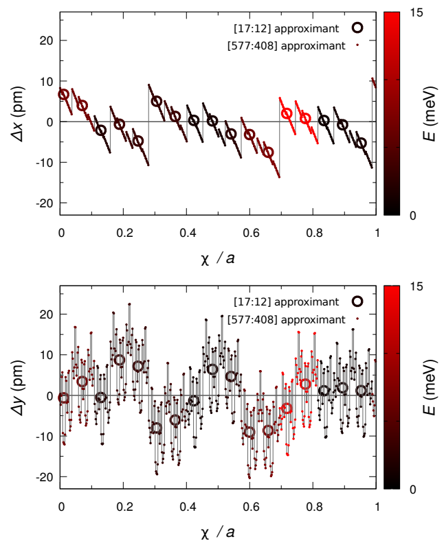
FIG. 10. Hull plots of the first atomic row of grain I at the incommensurate interface (see row iii of the lower grain in figure 9). The lattice parameter a is also the periodicity \ell of grain II. Top : atomic relaxation \Delta x along the incommensurate direction. Bottom : relaxation \Delta y perpendicular to the interface. The \Delta y origin corresponds to the average of the y coordinates in row iii . These hull plots are calculated with 17 Si atoms of the [17:12] approximant (large circles) and 577 atoms of the [577:408] approximant (small dots). Function discontinuities cannot be revealed by inspecting the [17:12] results. However, note that the atomic relaxations of the [17:12] approximant are representative of those of the [577:408] one, the small-model data following the trends of the large-model ones. The discontinuities and the apparent fuzziness of the [577:408] curves are intrinsic to this type of incommensurate interface. The curves could be continuous for another material, but here they are discontinuous everywhere. It is a pinned-state characteristic 42 .
