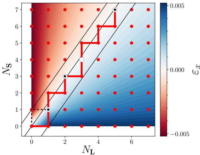
FIG. 7. Density plot of the strain \varepsilon_{x,II} in grain II for sequences made of N_L tiles \mathbf{L} and N_S tiles \mathbf{S} due to the misfit between the periodicities along the incommensurate direction of the two crystalline grains (see equations Eq. 3). Strain \varepsilon_{x,I} in grain I is the opposite. The red line (bold polygonal curve) represents \mathbf{S}_3 = \mathbf{LSSLSLSSLSLS} (Eqs. 4), a sequence that minimizes the strain field locally and on average.
