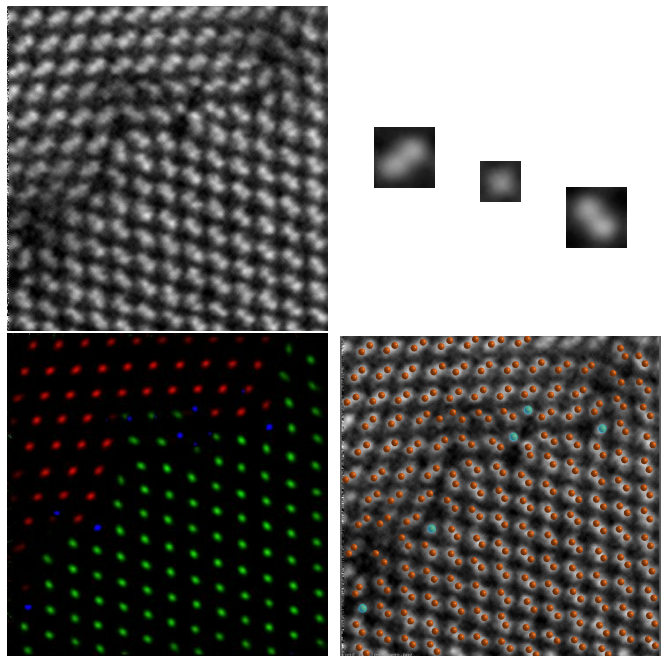
FIG. 3. (Color online) Illustration of the pattern recognition technique. (Top-left) Small part of an image, with grain II on top of grain I. (Top-right) Three patterns corresponding to grains I, II, and to isolated atomic columns. (Bottom-left) Color image representing the three correlation functions corresponding to the three patterns. Each correlation function represents one component of the RGB image coding (red-green-blue). A gamma correction of 4 has been applied to enhance the highest values of the correlations, i.e. , a power-law function with exponent 4 is applied to the components (normalized between 0 and 1). (Bottom-right) x and y atomic positions obtained by fitting, in the first image, individual or paired Gaussian functions, initially located at the maximum of the correlation functions. The individual atomic columns are distinguished by the color cyan.
