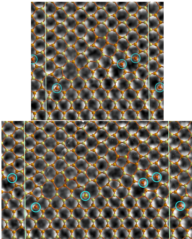
FIG. 4. (Color online) Electron microscopy images overlaid by the atomic configurations of the 5:7 and 10:7 approximants stable with the Stillinger-Weber interactions (respectively top and bottom images). For the bottom image, two images has been combined to get a sharper contrast. The light vertical lines indicate the periodicity along the interface. The coordinates z perpendicular to the images are color coded from red (lower z ) to yellow (higher z ). All Si atoms are tetra-coordinated. Atoms connected by bonds orthogonal to the images are surrounded by cyan circles.
