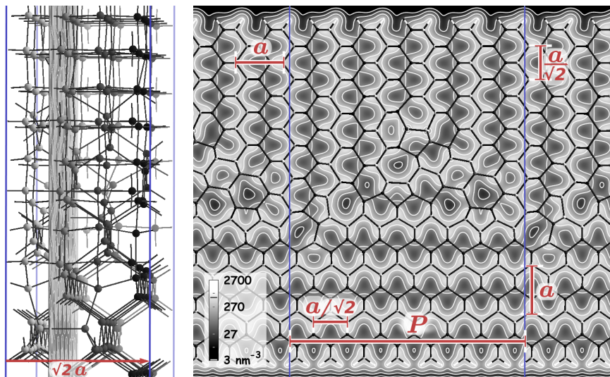
FIG. 5. Cross-section of the valence-electron density and ball-and-stick model of the 5:7 approximant. White and black in the grayscale represent respectively the highest and the lowest electron density. Left : Oblique view showing the location of the cross-section, which is perpendicular to the commensurate direction of the interface (common [1\bar{1}0] direction). Along this direction, the periodicity of the structure is \sqrt{2}a , where a is the cubic lattice parameter of silicon. Right : Plane view. The horizontal axis is the [001] direction of the upper grain and the [110] direction of the lower one. It is the opposite for the vertical axis. Along the incommensurate direction, P is the periodicity of the approximant. The logarithmic scale of the density plot is indicated by the gray-scale bar. The average density is N_e/V = 196 \text{ nm}^{-3} . The lattice parameter a = 547 \text{ pm} gives the length scale. The free-surfaces are passivated by hydrogen atoms.
