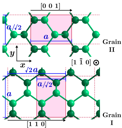
FIG. 1. Crystalline grain orientations on both side of the grain boundary. The Miller indices are relative to the cubic cell. The plan view is perpendicular to [1\bar{1}0] , which is the common direction of both grains ( z -axes here). The shades of the spheres indicate their altitude z = 0 or z = a/(2\sqrt{2}) . The light-shade rectangles of sides a and a/\sqrt{2} represent the silicon orthorhombic cells with the lattice vectors corresponding to [001] , [110] , and [1\bar{1}0] . The cubic cell is projected onto (1\bar{1}0) as a rectangle of sides a (side of the cube) and \sqrt{2}a (diagonal of the face). The vector [001] of one of the crystal is parallel to the vector [110] of the other one, and thus the grain boundary is incommensurate. In this study, the interface is parallel to the xz -plane.
