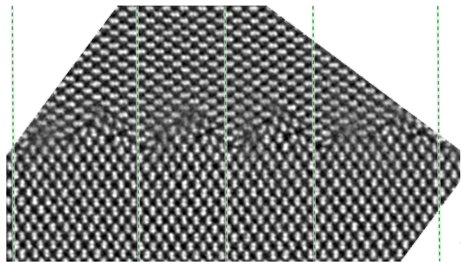
FIG. 2. Scanning transmission electron microscopy (STEM) image of the incommensurate grain boundary. Si atoms, individual or in adjacent pairs (dumbbells), are all resolved in this image. More precisely, each spot corresponds to an atomic column perpendicular to the plane view. Vertical lines indicate a possible decomposition into 7:5 and 10:7 approximants of the grain boundary (thinner and thicker strips, respectively). Note the good atomic match between atomic patterns at the different line locations making possible periodic boundary conditions for each approximant, or combinations of several 7:5 and 10:7 approximants.
