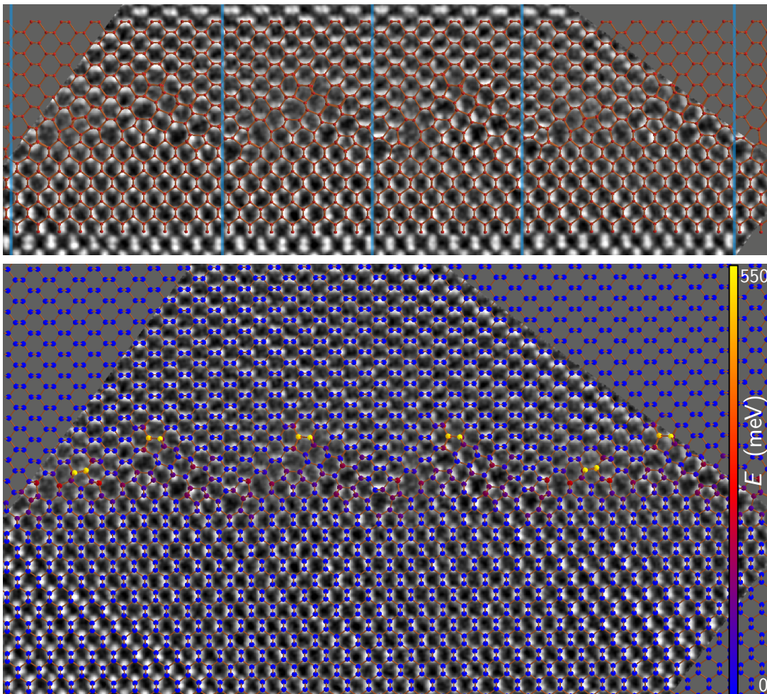
FIG. 8. Top: Overlay of the experimental image by a sequence of \mathbf{S} and \mathbf{L} tiles, i.e. respectively the [7 : 5] and [10 : 7] approximants, each one calculated by DFT. The vertical lines indicate the tile boundaries. Bottom: Overlay of the experimental image by a [41 : 29] approximant corresponding to the sequence \mathbf{S}_2 , now relaxed with the Stillinger-Weber potential 23 . The energy of the atoms with this potential is color coded (online version) from blue (bulk energy) to red and yellow (highest energy). Note that the image contrast is correlated with the atom energies: when a high energy has been found the contrast is lower, probably indicating structure perturbations like a higher vacancy concentration or larger atomic moves.
