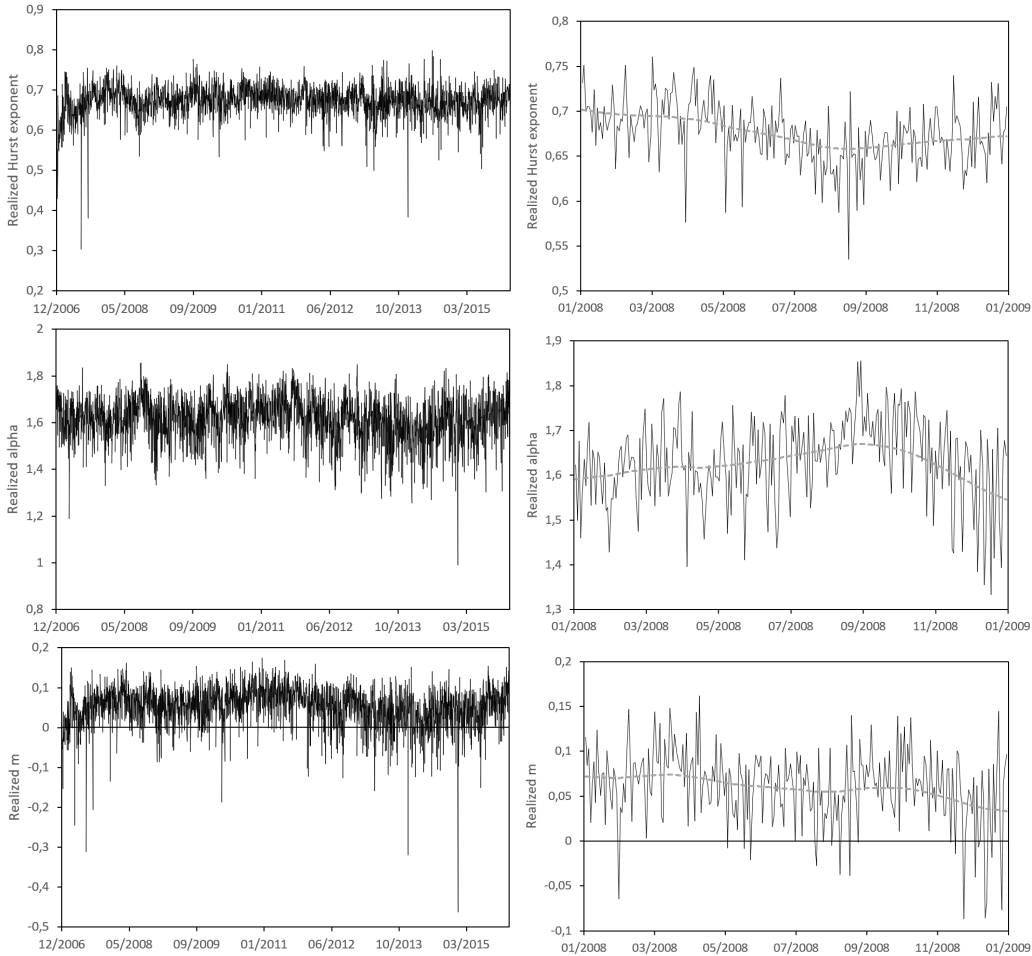
Figure 2: Daily estimates of H , \alpha , and m , for the EUR/GBP pair, between December 2006 and January 2016 (left), and in 2008 (right). The dotted line is a smooth approximation obtained by variational smoothing.
