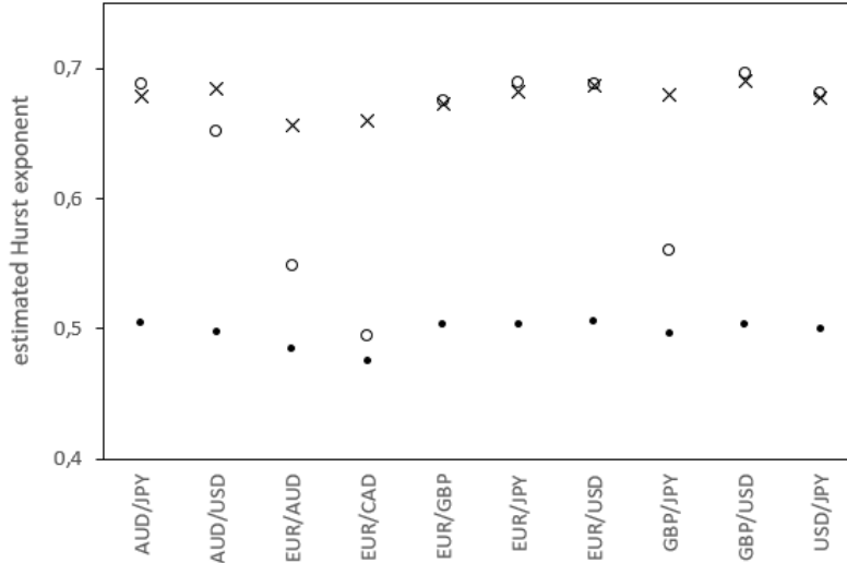
Figure 3: Average realized Hurst exponents (crosses) and estimated global Hurst exponents using the regression on the 200 lowest scales (dots) or the 2 lowest (circles).
