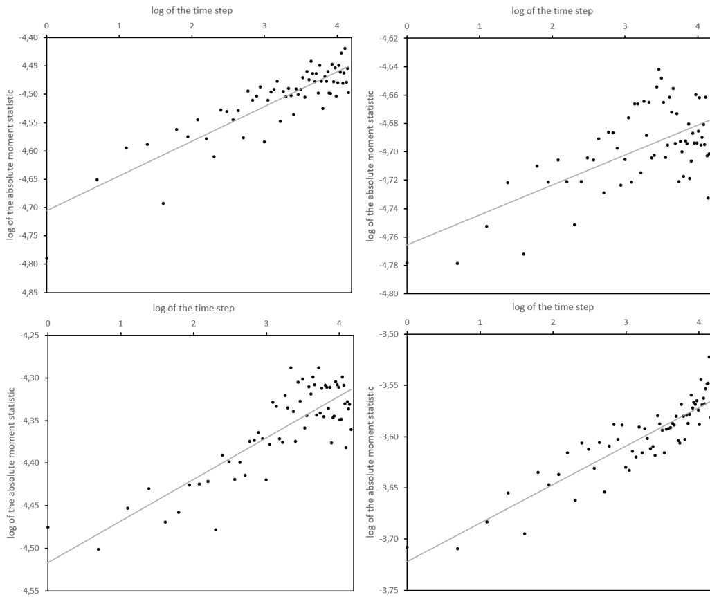
Figure 4: Empirical log plot of the series of realized Hurst exponents for EUR/JPY (top left), EUR/USD (top right), EUR/GBP (bottom left), and GBP/JPY (bottom right). Half the slope of the corresponding affine regressions (in grey) is the estimated Hurst exponent of the Hurst exponents.
