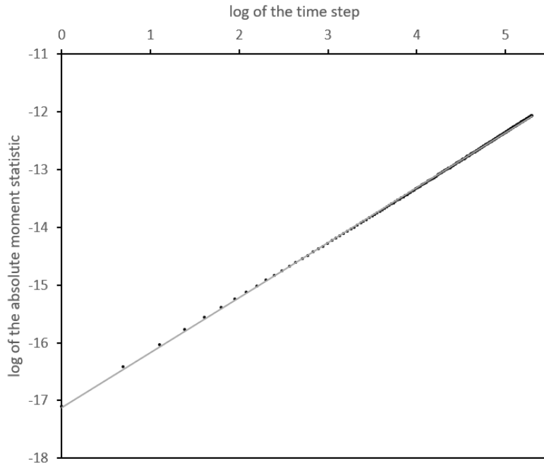
Figure 1: Empirical log plot for the EUR/CAD series, with the corresponding affine regression in grey. We estimate the Hurst exponent by half the slope of the regression.
