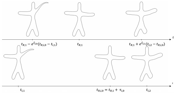
Fig. 3 Example of a time reparametrization. At the top, the representative trajectory. At the bottom, a time reparametrization towards the subject i observed at two times: t_{i,1} and t_{i,2} . The individual rupture time of the subject i is obtained as a translation of the rupture time by \tau_{i,0} , here chosen positive. On the first time segment, \xi_{i,0} is negative and the progression is slower than the one of the representative trajectory. On the second time segment, \xi_{i,1} is positive and the progression is quicker.
