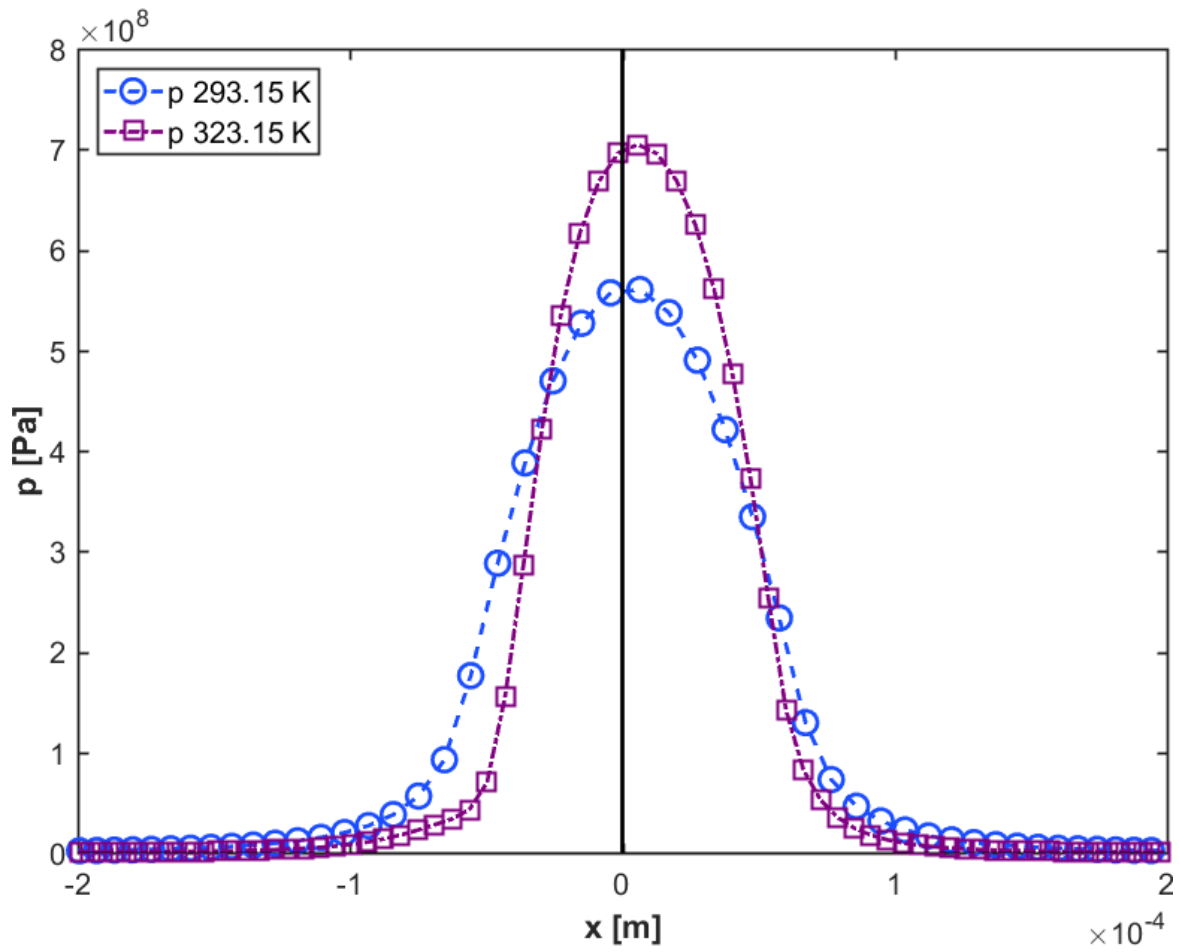
Figure 12 – Pressure profiles at u = 5 m/s and w^{1D} = 5.82 \times 10^4 N.m -1 , for two different external temperatures.
