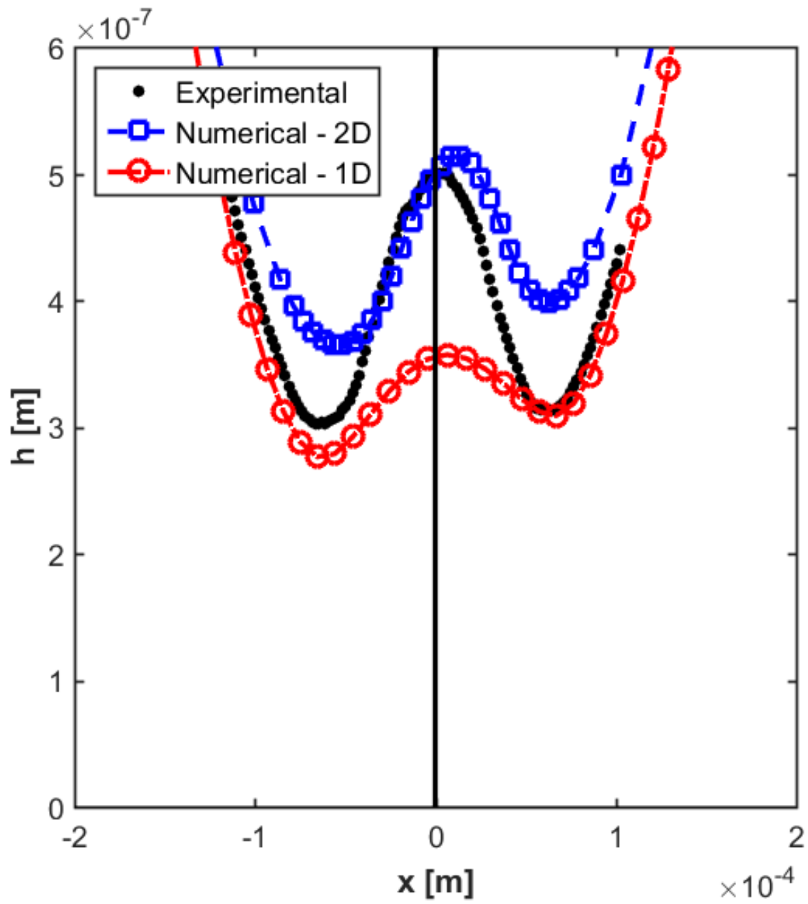
Figure 3 – Film thickness profiles for the reference case ( u = 5 \text{ m/s} , w^{2D} = 50 \text{ N} or w^{1D} = 5.82 \times 10^4 \text{ N}\cdot\text{m}^{-1} and T_0 = 293.15 \text{ K} ), from experiments (along the dashed line in Figure 2) and simulations.
