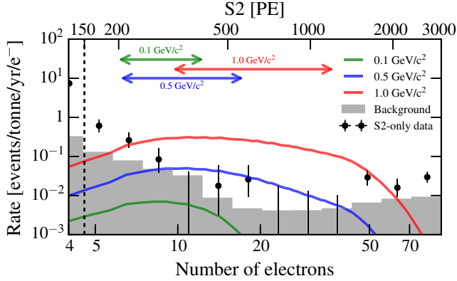
FIG. 4. Observed S2 spectra for the S2 -only data after the optimized selection described in Ref. [21]. The expected spectra of ER signals induced by MIGD for DM with mass of 0.1, 0.5, and 1.0 \text{GeV}/c^2 are shown in green, blue, and red solid lines, respectively, assuming the spin-independent DM-nucleon interaction cross section of 1.2 \times 10^{-37} , 1.5 \times 10^{-39} , and 2.0 \times 10^{-39} \text{ cm}^2 for 0.1, 0.5, and 1.0 \text{GeV}/c^2 DM, respectively. The gray shaded region shows the conservative background model used in analysis of S2 -only data. The arrows indicate the S2 ROIs that are later used in inference for the three DM signals mentioned above. The S2 threshold used for the S2 -only data is denoted in the dashed black line.
