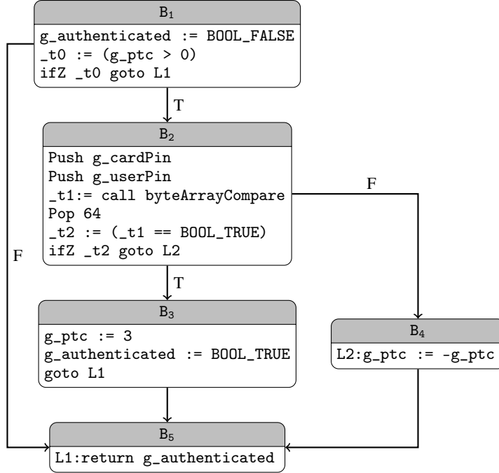
Figure 2: CFG for the verifyPIN function.
