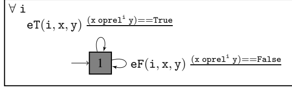
Figure 3: M_{IT} , a QEA detecting test inversion attacks.
