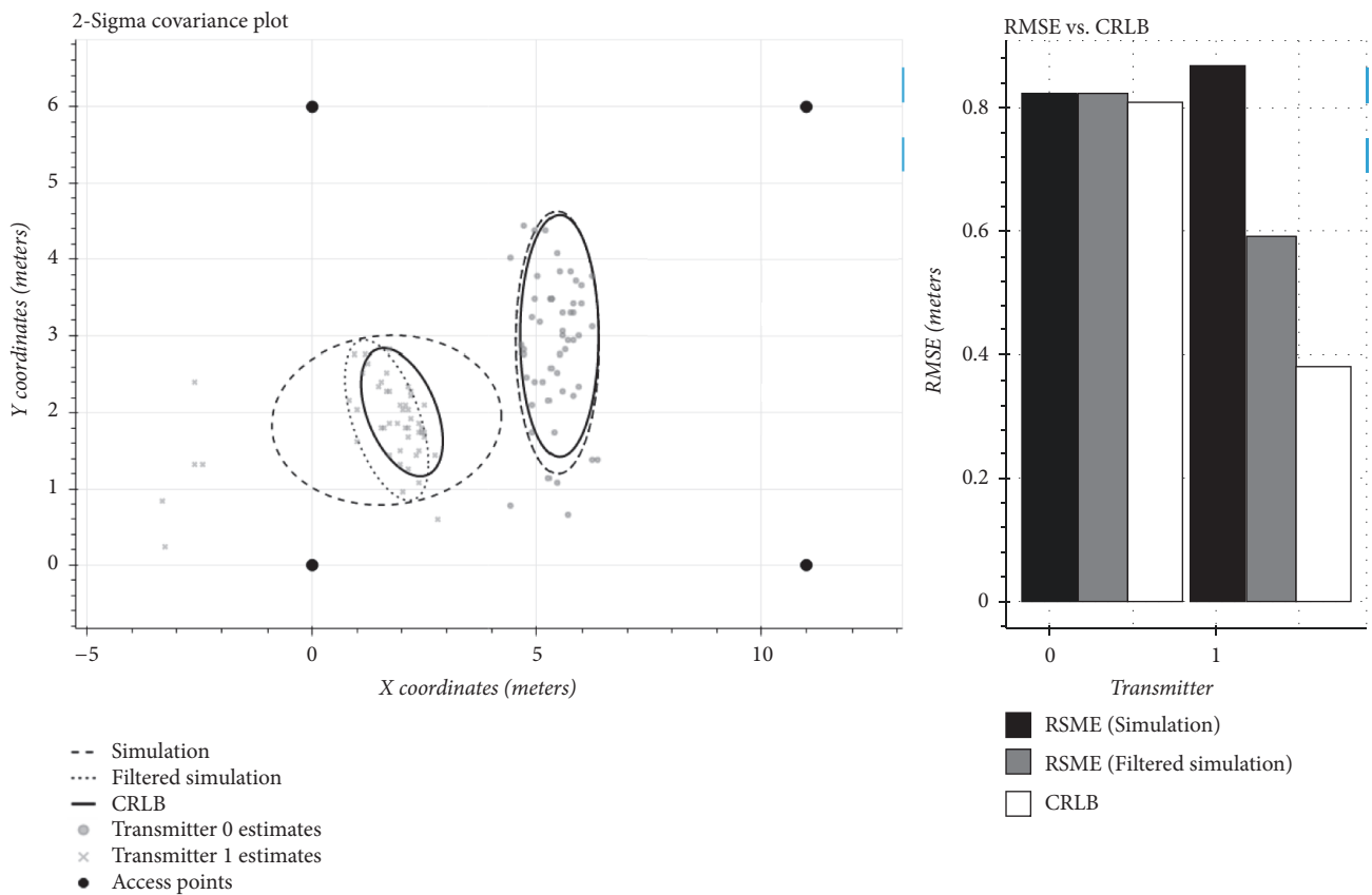
FIGURE 1: Numerical verification of the CRLB equation. The left figure shows 2-sigma covariance of simulated position estimates using MLE estimator vs. the covariance from our CRLB expression. Right figure shows the RMSE from simulation data and the CRLB trace.
