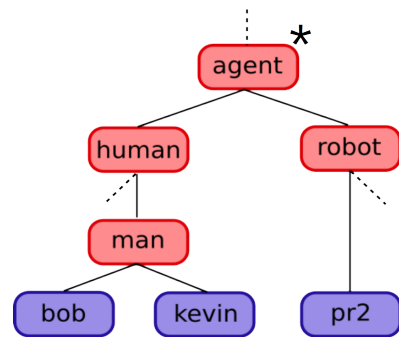
Fig. 7: Inheritance relations of the concepts "Bob", "Kevin" and "Pr2". The class "agent" (*) represents the common point between the three concepts.
