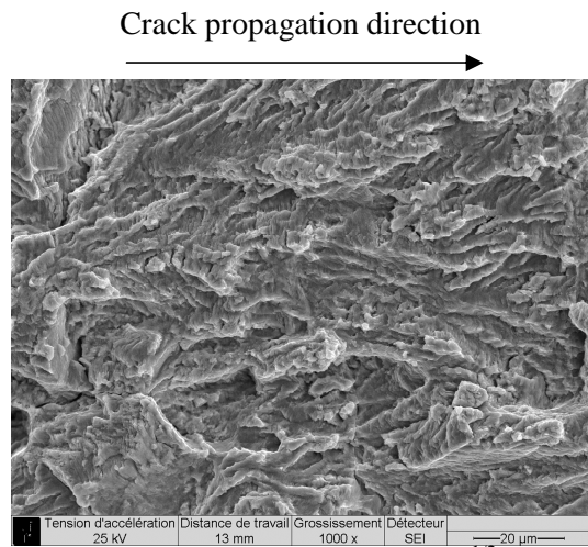
(b) At \Delta K = 15 \text{ MPa}\times\text{m}^{1/2}
