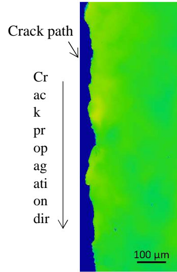
(b) At f = 0.2 Hz in hydrogen of P_{H_2} = 35 MPa.
