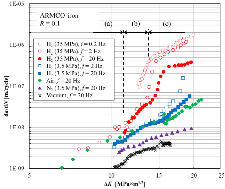
Fig. 2 FCGRs ( = da/dN ) vs \Delta K in Armco iron at various hydrogen gas pressures and loading frequencies [23,31].
