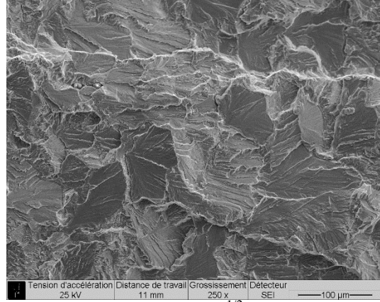
(b) At \Delta K = 18 \text{ MPa}\times\text{m}^{1/2} and f = 20 \text{ Hz} .
