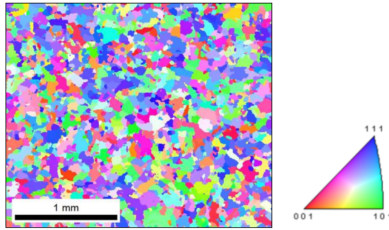
Fig. 1 EBSD mapping of the microstructure of Armco iron used in this study. The average grain size is about 90 \mu\text{m} .
