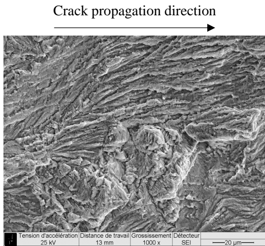
(a) At \Delta K = 8 \text{ MPa}\times\text{m}^{1/2}
