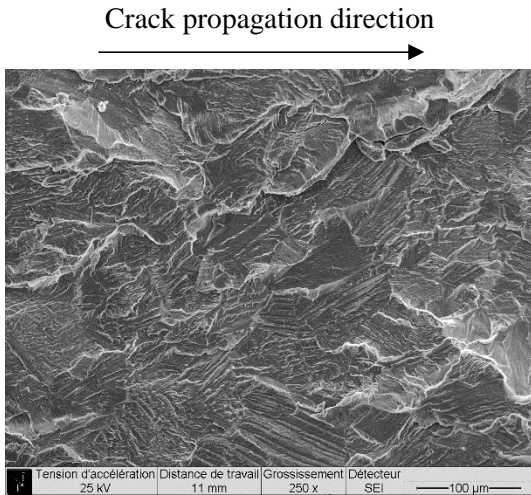
(c) At \Delta K = 18 \text{ MPa}\times\text{m}^{1/2} and f = 0.2 \text{ Hz} .
