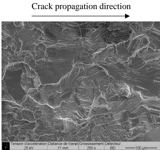
(e) At \Delta K = 18 \text{ MPa}\times\text{m}^{1/2} and f = 20 \text{ Hz} .
