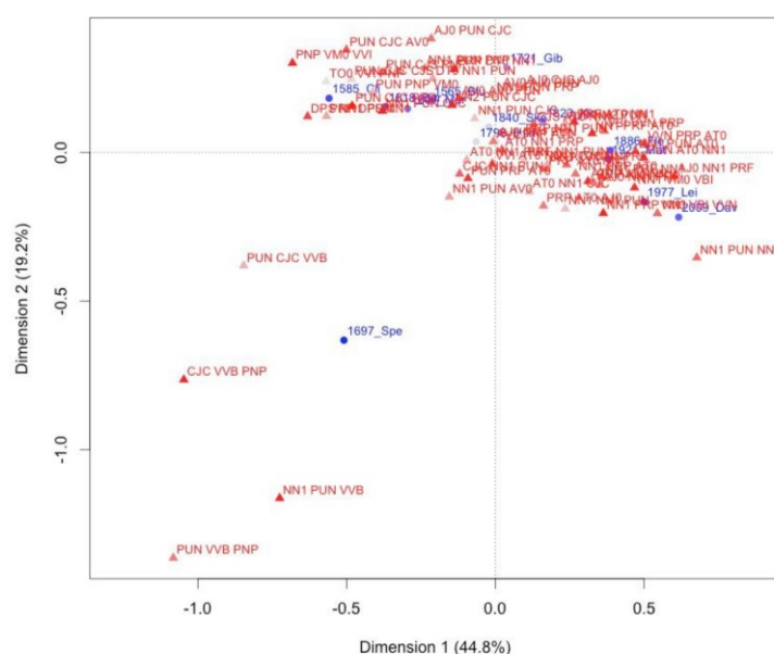
Figure 3. Symmetric plot of trigrams and sources (100+ observations).
