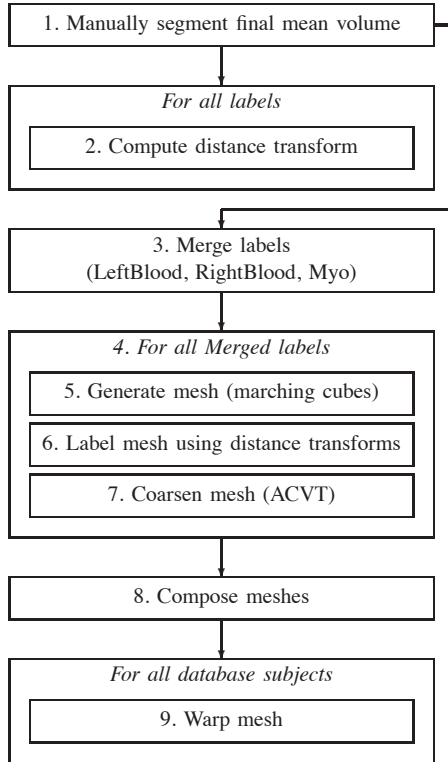
Fig. 4. Flow diagram of the meshing steps. ACVT: Approximate Centroidal Voronoi Tesselation. Initially the nine labels are merged into three; using the nine distance transforms, the vertices on the marching cubes meshes are labeled before coarsening. The atlas is finally composed by putting the three labeled, coarsened meshes together.
