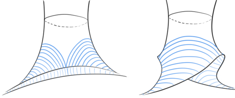
FIGURE 6. The partial horocyclic foliation on S - \mu , viewed from two different perspectives.
