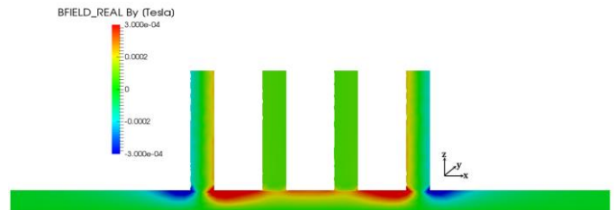
Fig. 9. Magnetic induction along the y axis ( f=5\text{Hz} , \mu_r=5 )
