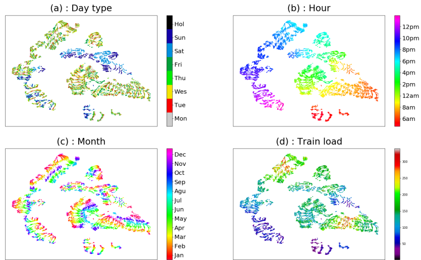
Fig. 7. Latent representation ( \mathbf{u}_t ) according to contextual features obtained after dimensionality reduction (PCA + tSNE)
