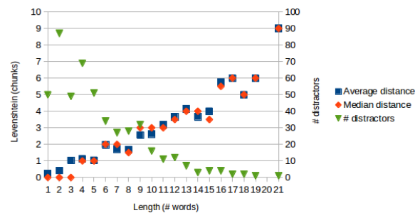
Figure 2: Levenshtein distance between chunks of distractors and their associated answers according to lengths of distractors, and number of distractors per length
