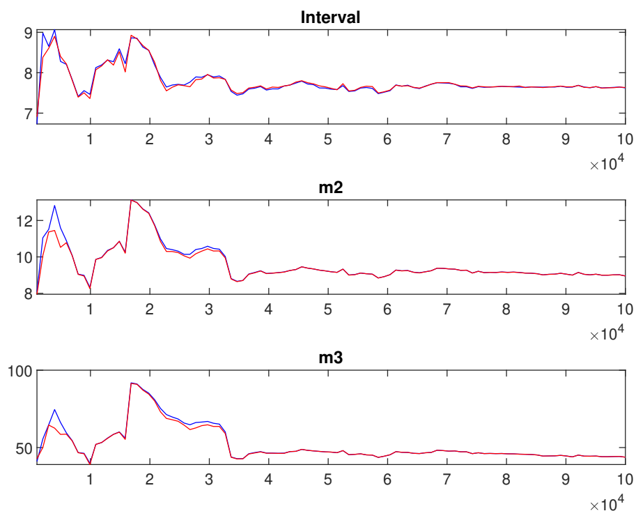
Figure 2: Multivariate Convergence Diagnostic: Nominal GDP Targeting Rule
