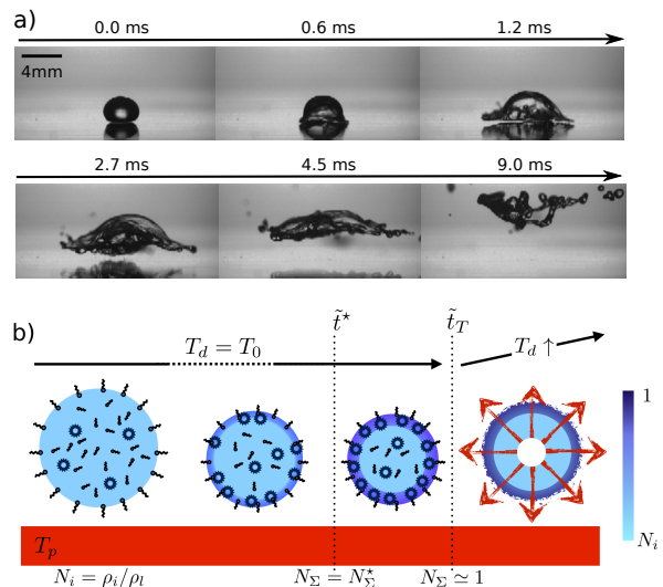
FIG. 1. a. Example of an explosion of a droplet. Initial size of the drop 100 \mu\text{L} , initial concentration 10 CMC and temperature of the plate 400^\circ\text{C} . b. Schematic representation of a droplet life. To begin with, free molecules and micelles are uniformly distributed. During the evaporation, the droplet shrinks and micelles accumulate at its surface, leading from \tilde{t} = \tilde{t}^* to the formation of a gel-like shell. From \tilde{t} = \tilde{t}_T the temperature of the droplet, T_d , rises above the boiling temperature T_0 , leading to vapor bubble nucleation, growth, shell stretching and finally explosion of the droplet. N denotes the SDS mass fraction and \rho the density (with subscripts i , l and \Sigma for “initial”, “liquid” and “surface”, respectively).
