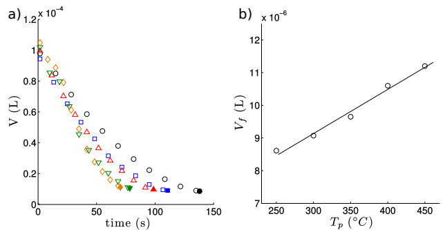
FIG. 3. a. Volume vs time for water/SDS droplets at several temperatures of the plate: \circ 250°C \square 300°C \triangle 350°C \nabla 400°C \diamond 450°C. Filled symbols are used for the final volume before the explosion. The initial concentration of the droplet is 10 CMC and the initial size of the droplet is 100 \mu\text{L} . b. The final volume before explosion, V_f is plotted vs the temperature of the plate T_p . The line is a linear fit.
