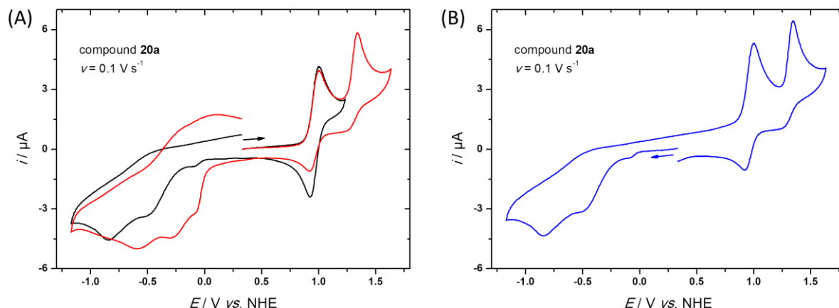
Figure 2. Cyclic voltammetry at a Pt electrode of compound 20a in \text{CH}_2\text{Cl}_2/\text{NBu}_4\text{PF}_6 0.1 M ( \nu = 0.1 \text{ V s}^{-1} , C = 0.5 \text{ mM} ); A) in positive initial scanning; B) in negative initial scanning. Experimental curves were measured against Fc and recalibrated by taking E^0(\text{Fc}^+/\text{Fc}) = 0.71 \text{ V vs. NHE} in those conditions.
