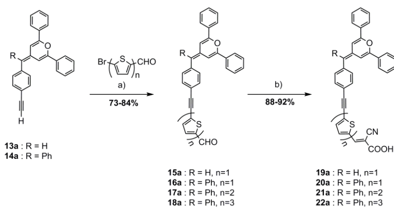
Scheme 3. Synthetic route of dyes 19a , 20a , 21a , and 22a . Reagents and conditions: a) \text{Pd}(\text{PPh}_3)_4 , \text{CuI} , THF, \text{NH}_4\text{Pr}_2 , 60^\circ\text{C} , overnight. b) Cyanoacetic acid, piperidine, \text{CHCl}_3 , reflux, overnight.
