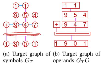
Fig. 1: The graph G_T generated with rules over the arithmetic operation: 954 + 947 .
