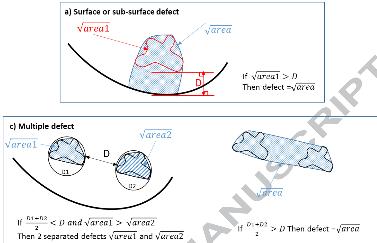
Figure 11: definition of the defect size depending on its location relative to the free surface, D1 and D2 are the diameters of a circles that encapsulates the corresponding defect.
